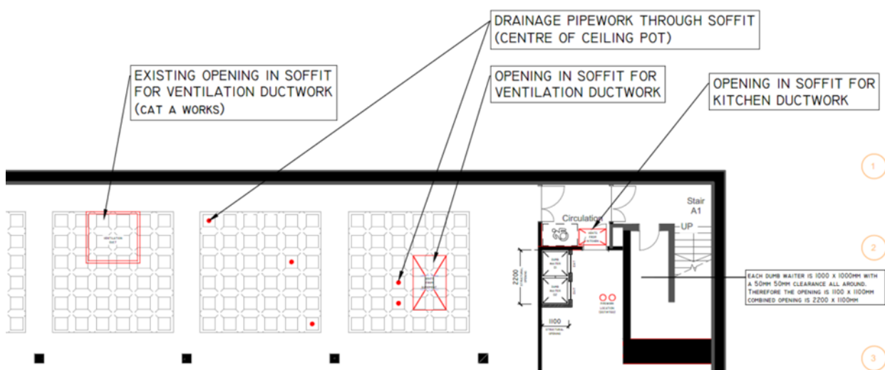
Figure 1: Ventilation openings – basement level (extract from drawing 4021-F00-008)
