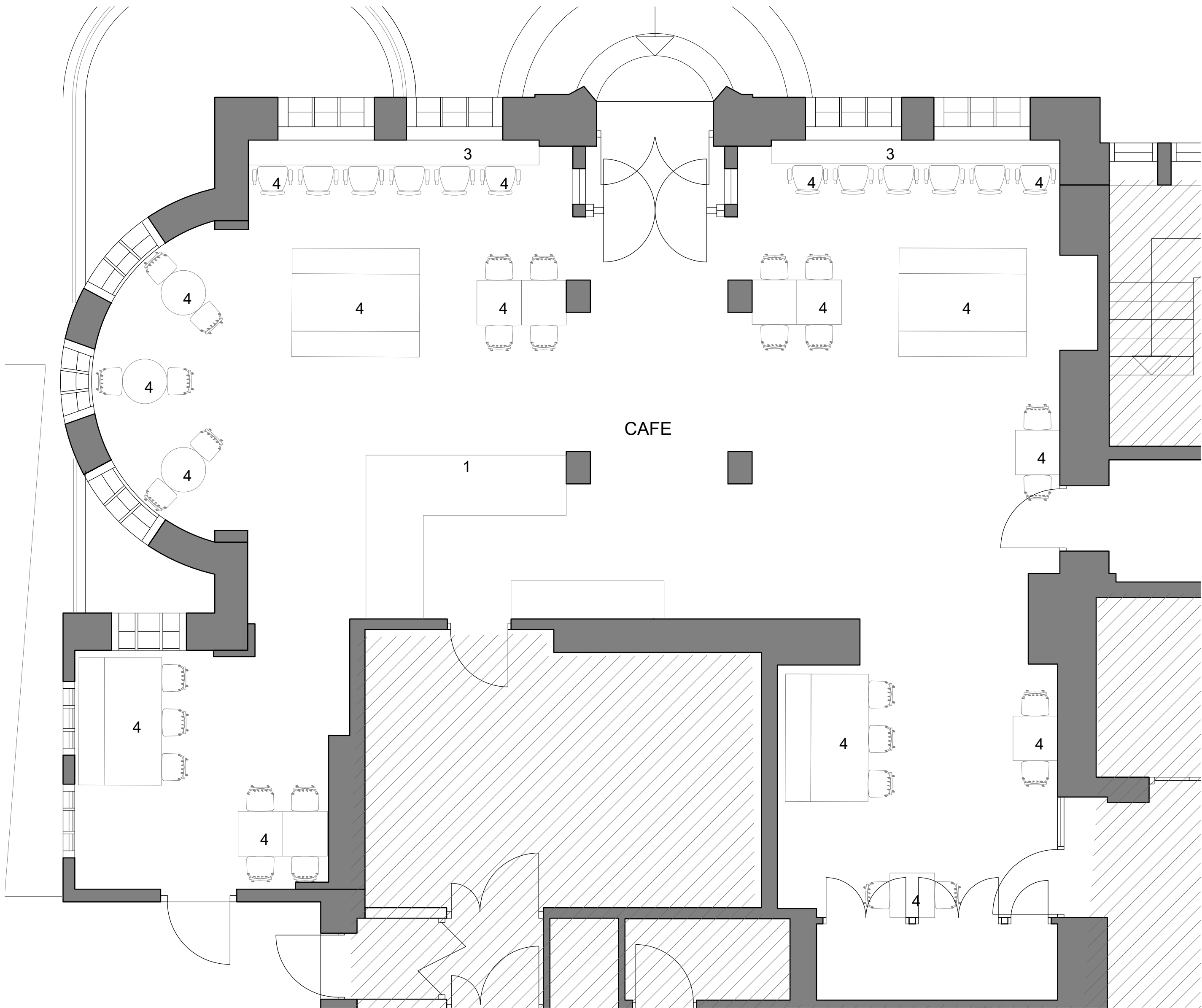
Ground Floor Proposed Plan - Cafe 1:50
