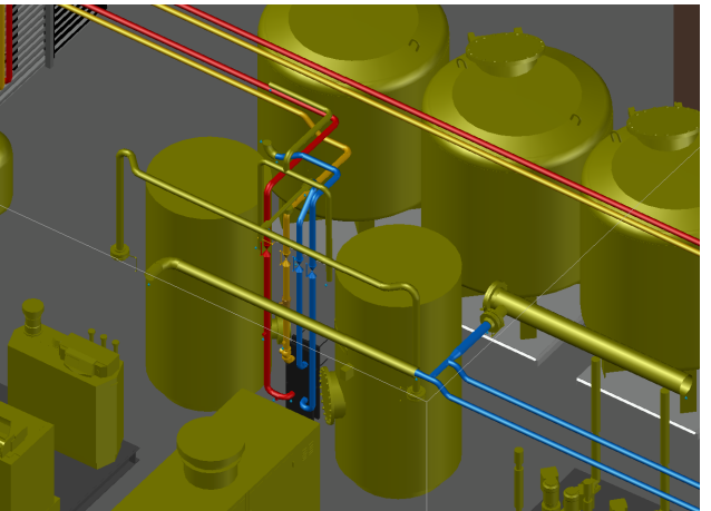
ISOMETRIC VIEW OF EXISTING DHW CALORIFIER BREAK-INS LOOKING NORTH-WEST SCALE 1:50
