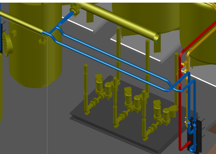
ISOMETRIC VIEW OF CHW HEATING CIRCUIT BREAK-IN LOOKING NORTH-WEST SCALE 1:50
