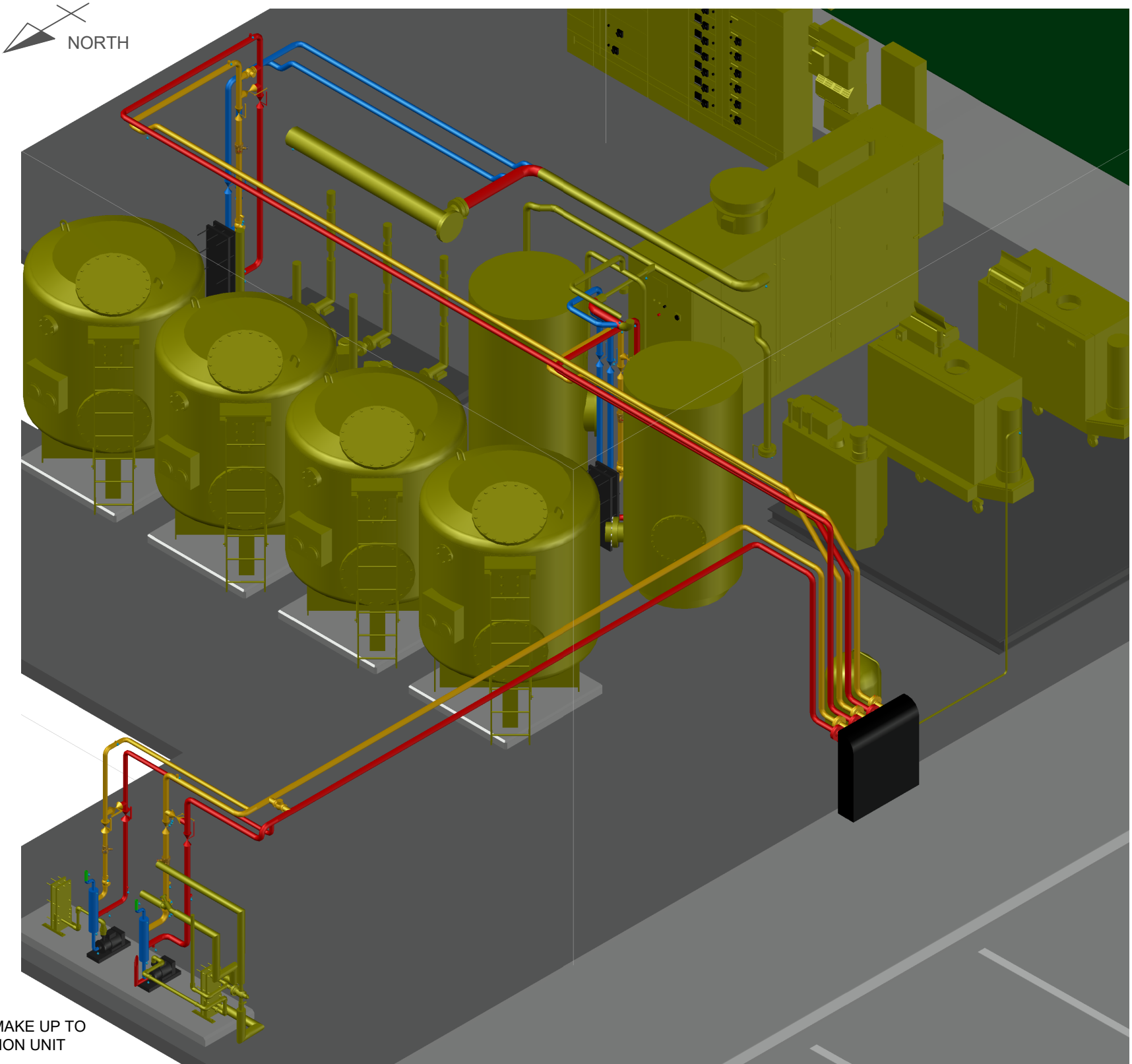
ISOMETRIC VIEW OF EXISTING PLANTROOM LOOKING SOUTH-EAST SCALE 1:50
