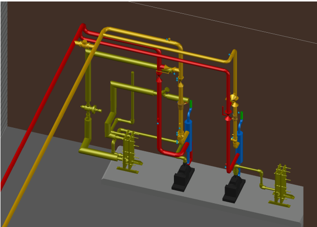
ISOMETRIC VIEW OF LEARNER AND MAIN POOL BREAK-INS LOOKING NORTH-WEST SCALE 1:50
