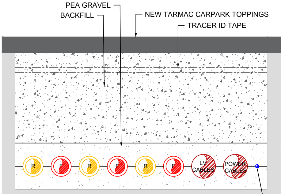
DETAIL 1: PIPEWORK & CABLE TRENCH VIEW LOOKING 'A'-A' N.T.S - REF TO EP2012D-05
