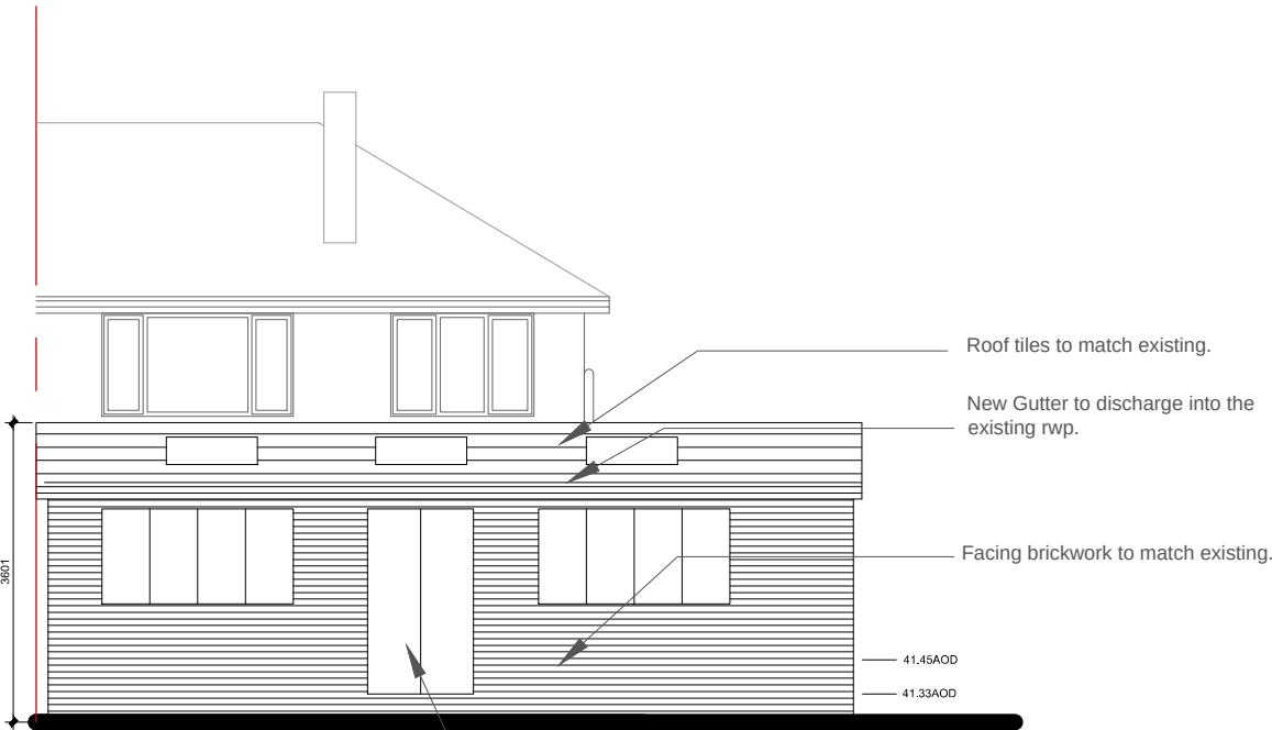
Rear Elevation
