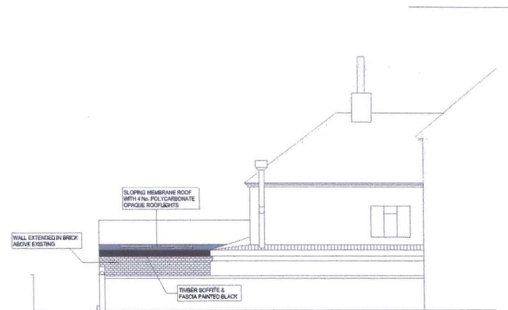
Side Elevation (North-West) - 1:50
