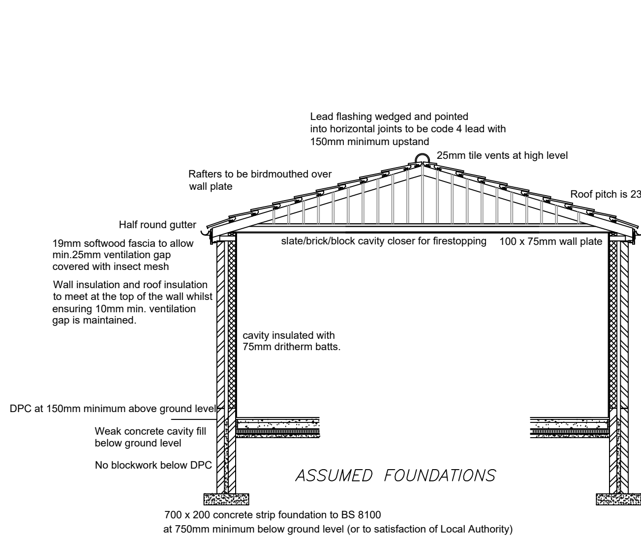
TYPICAL SECTION
