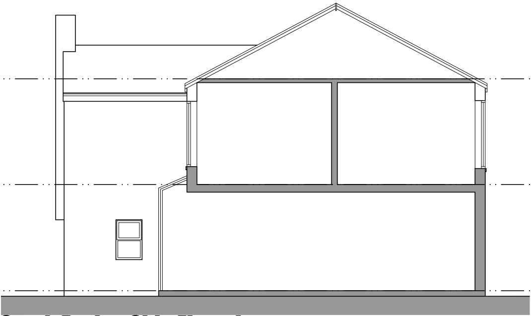
South Facing Side Elevation
