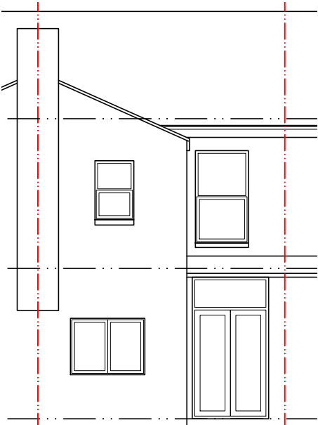
West Facing Rear Elevation
