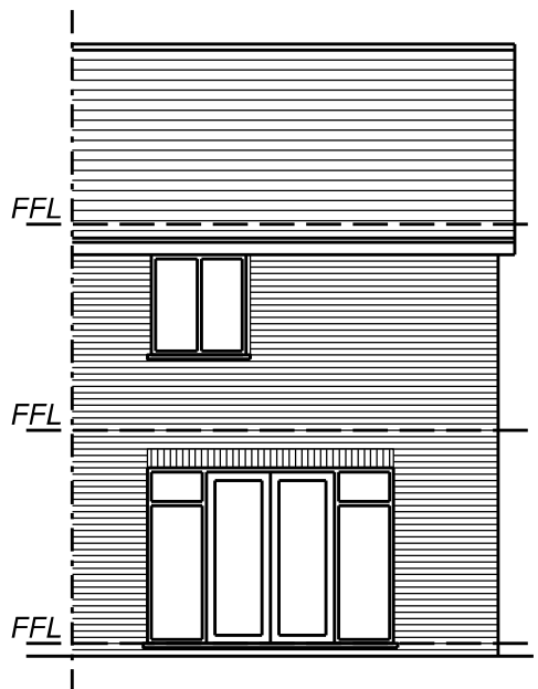
North Elevation
