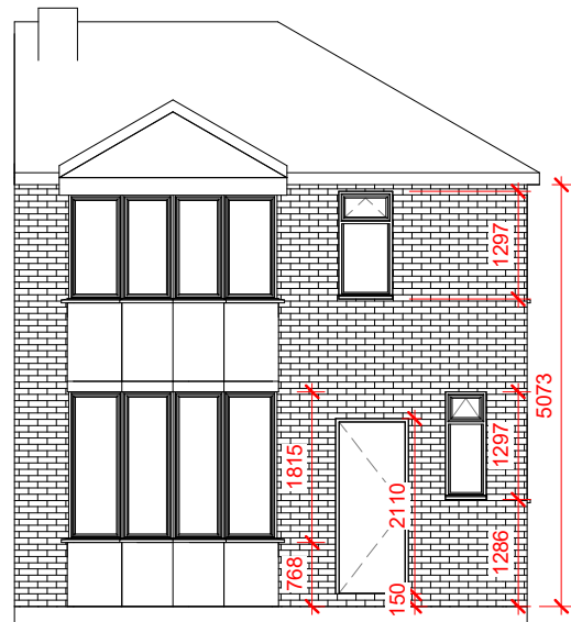
1 Front Existing 1 : 100
