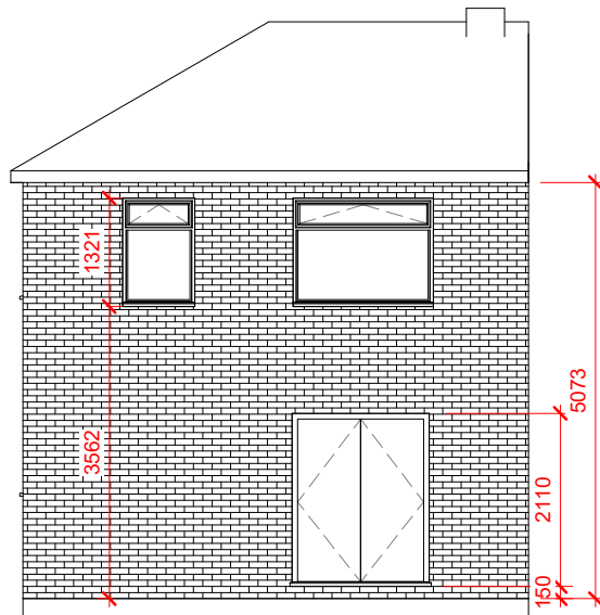
3 Rear Existing 1 : 100
