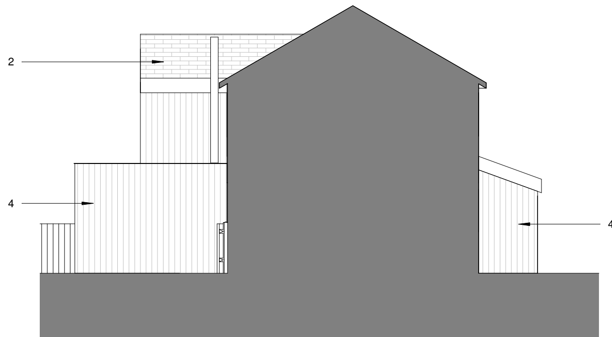
Proposed Elevation East no. 12 1 : 100
