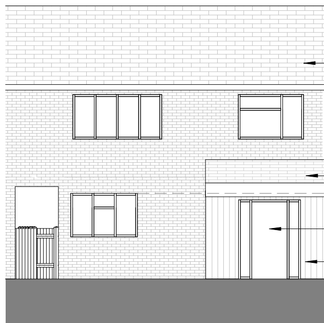
Proposed Elevation North no. 12 1 : 100
