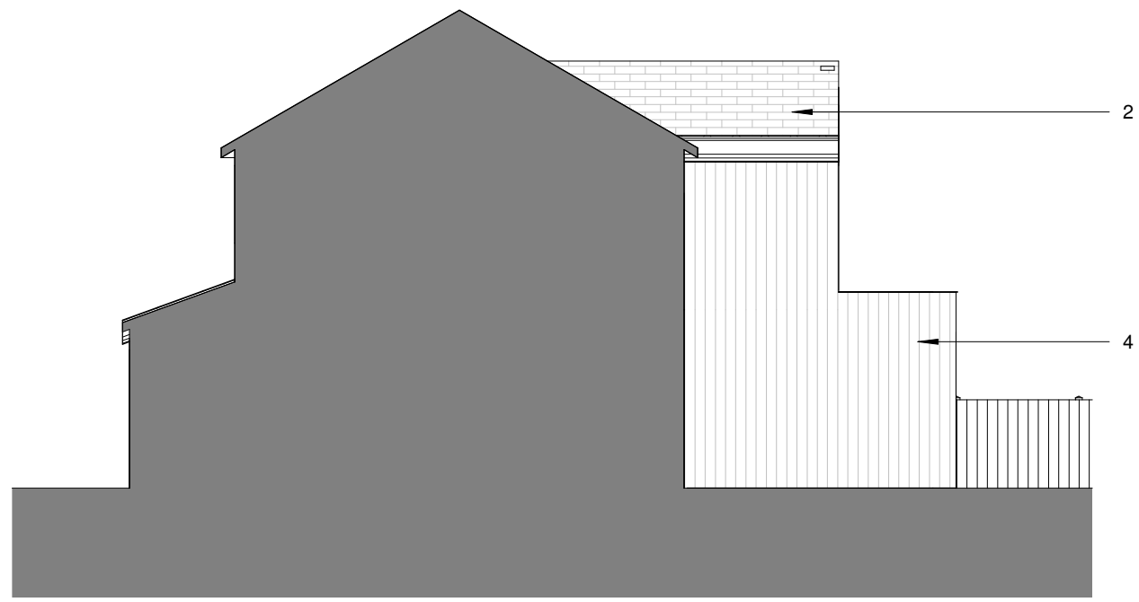
Proposed Elevation West no. 12 1 : 100
