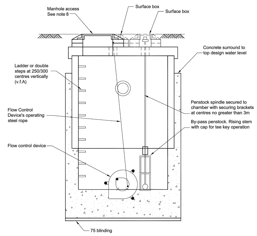
SECTION B-B
