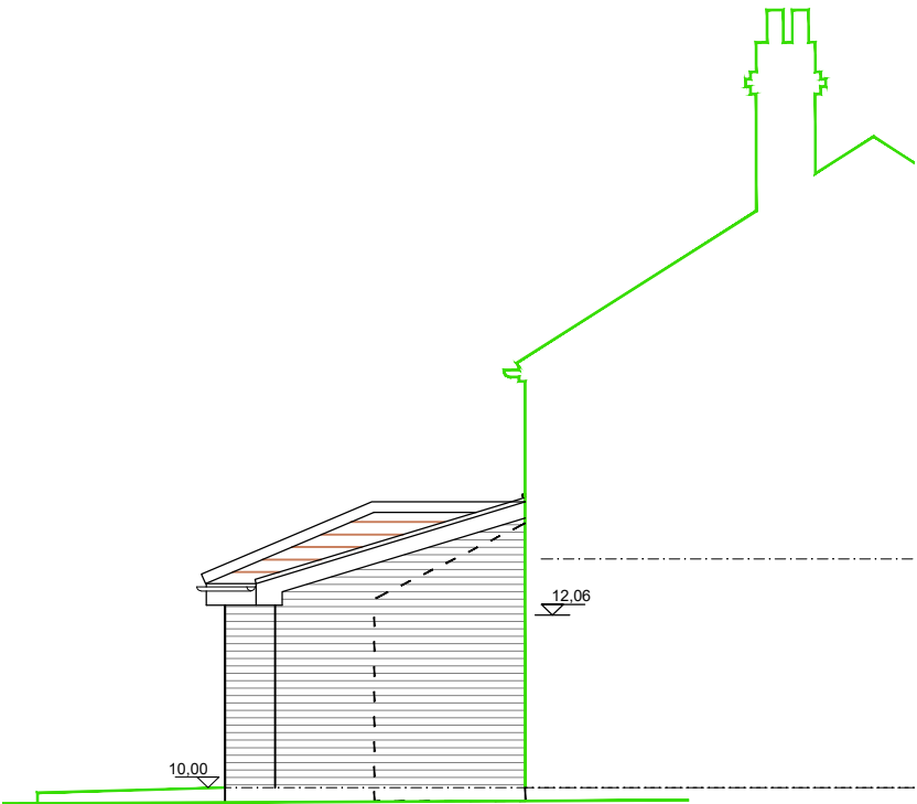
EAST ELEVATION
