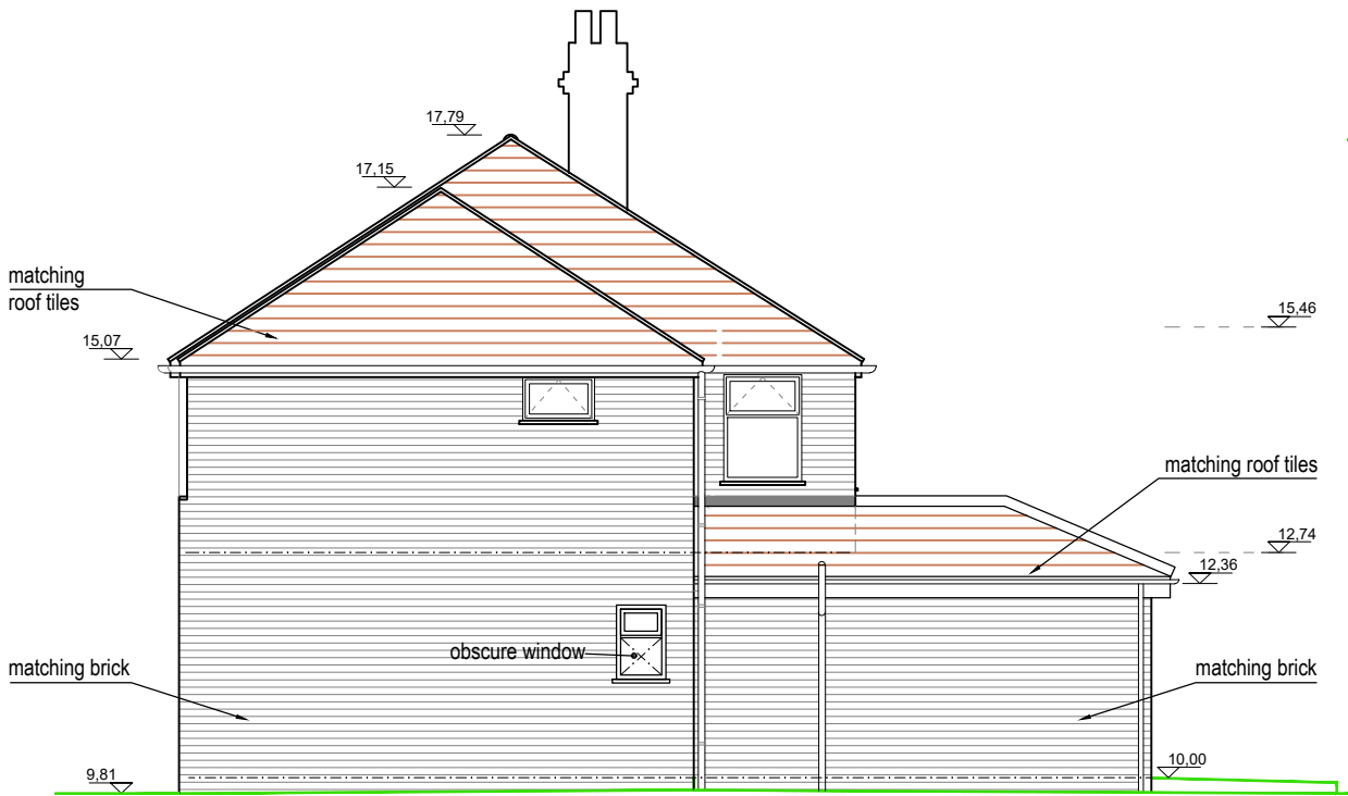
WEST ELEVATION
