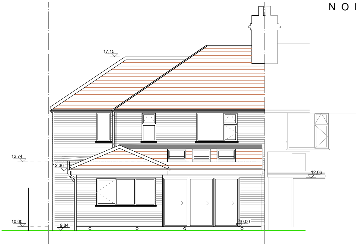
SOUTH ELEVATION
