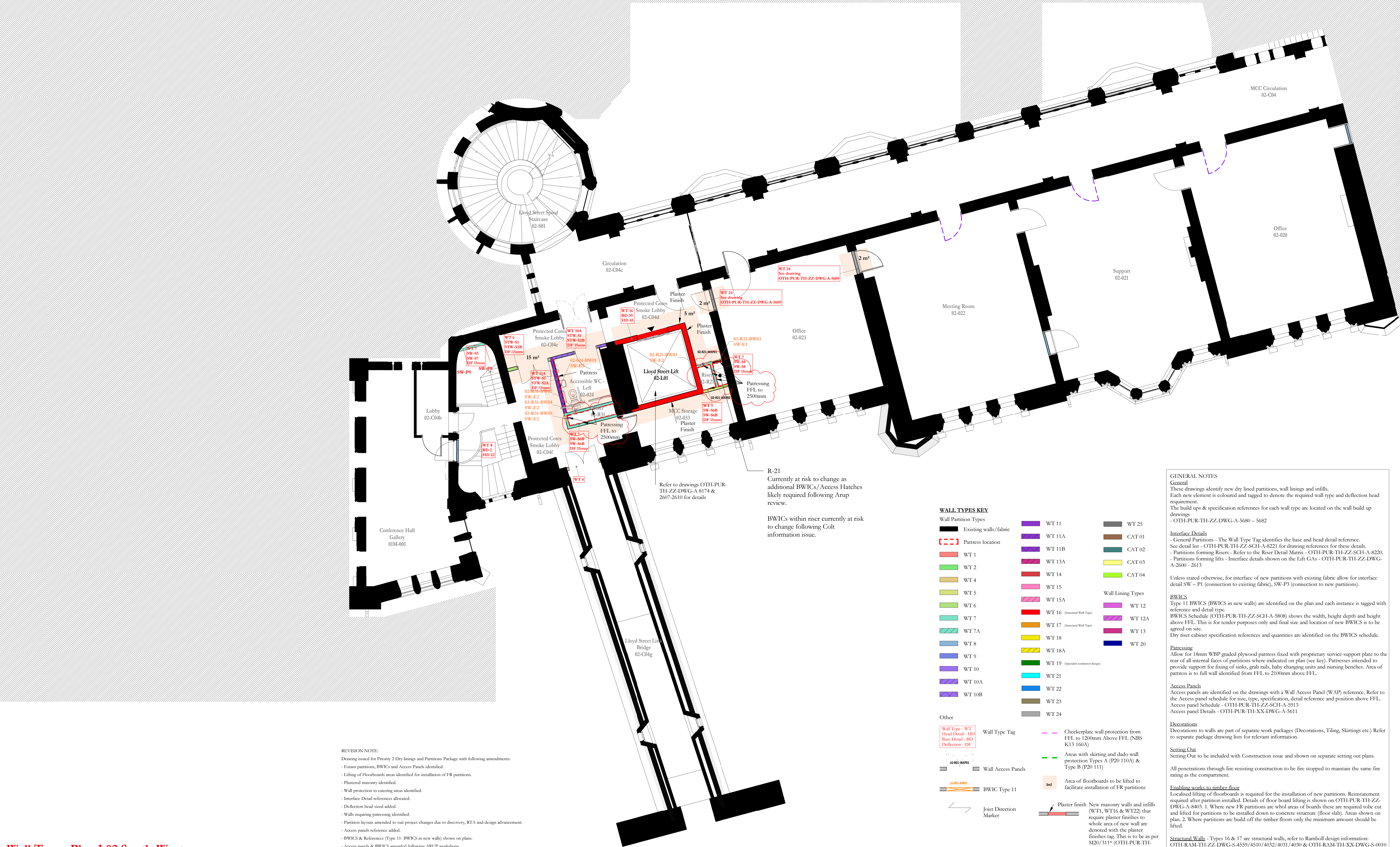
Wall Types Plan L02 South-West 1 : 100
