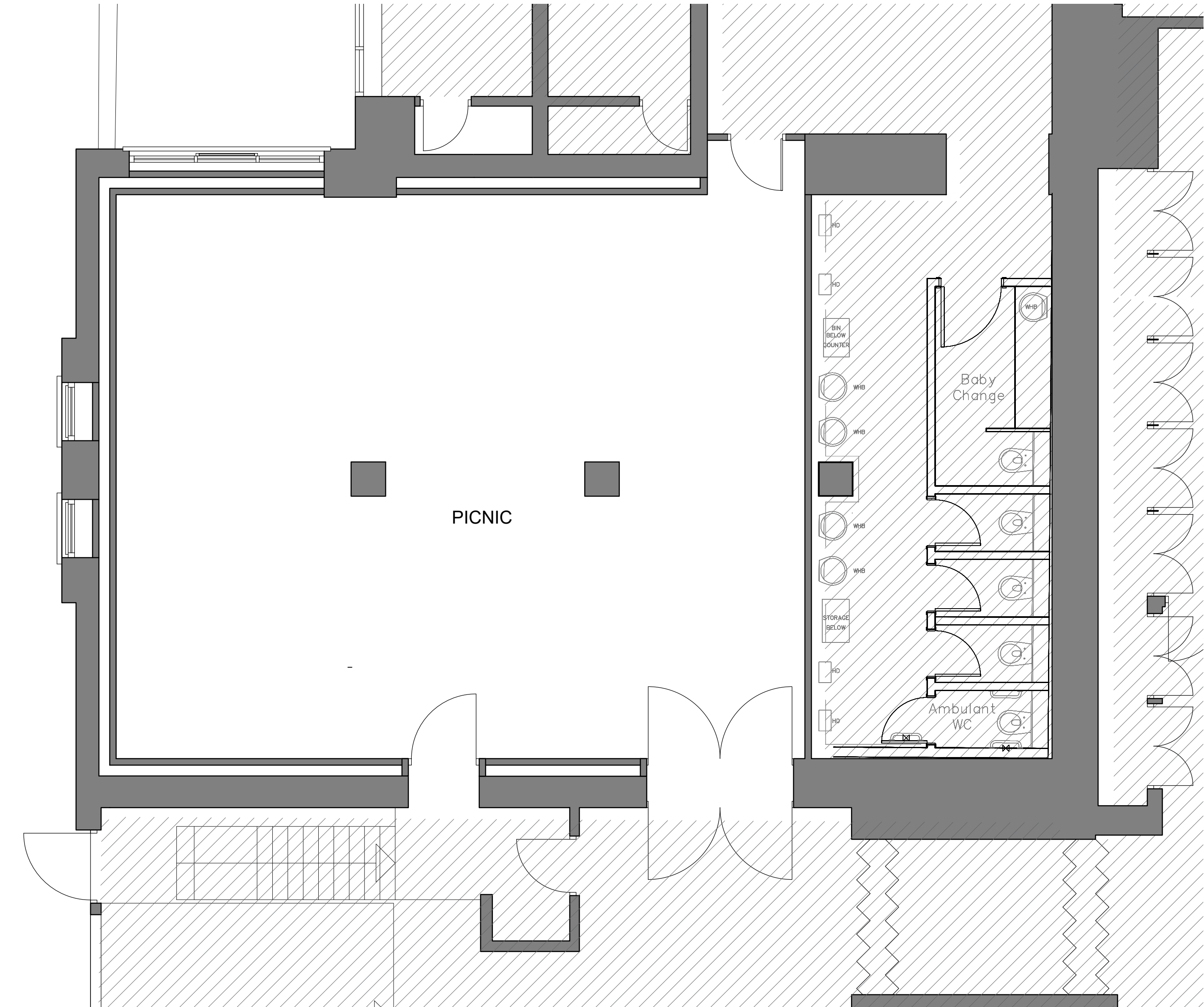
Ground Floor Existing Plan - Picnic 1:50
