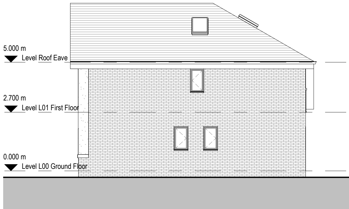
4 Existing North Elevation 1 : 100
