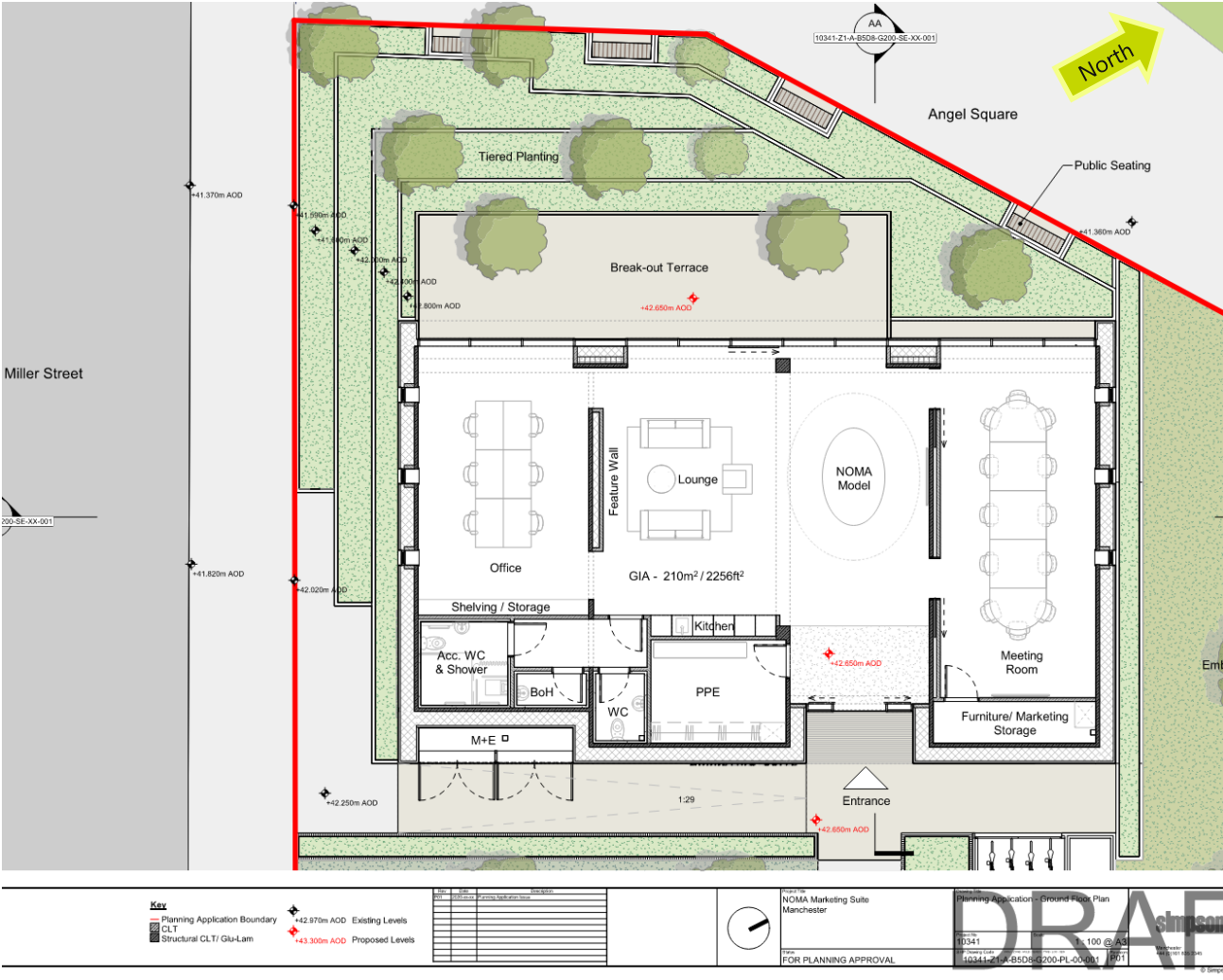
Figure 5—1 Plan of marketing suite, showing internal layout and external façade
