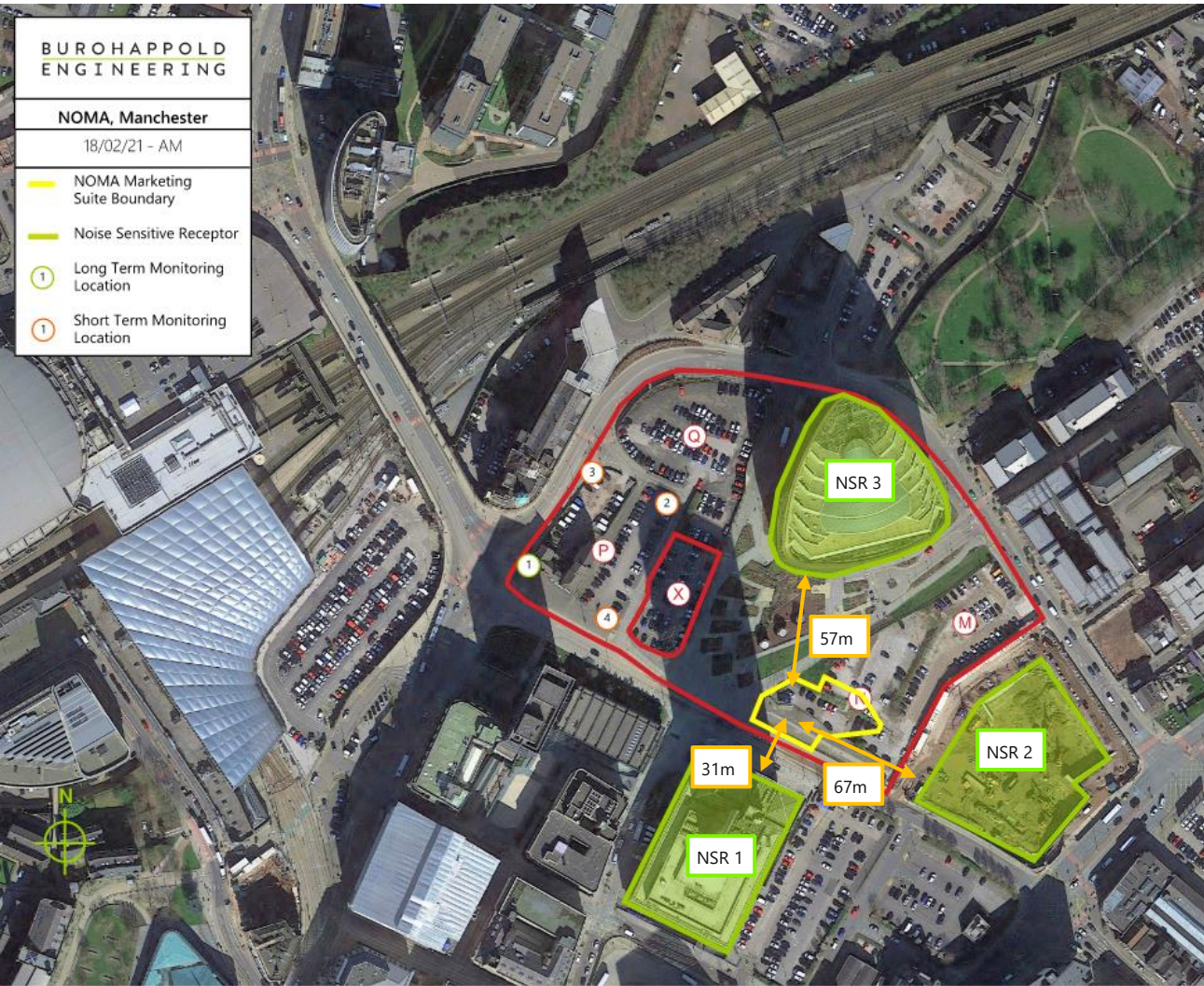
Figure 3—1 Site plan showing measurement locations, NSRs and site boundary
