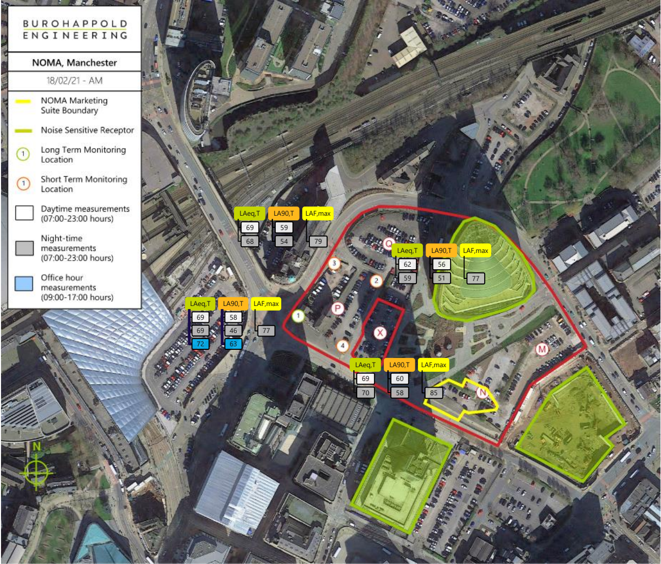
Figure 2—2 Site plan showing noise measurement summary
