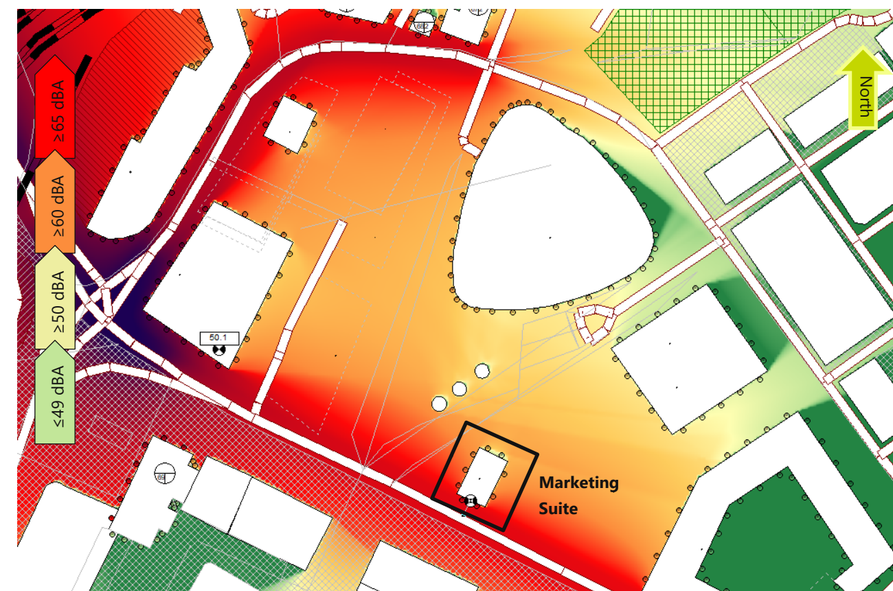
Figure 4—1 Plan view of predicted site wide noise levels during office hours ( L_{Aeq,T} dB)
