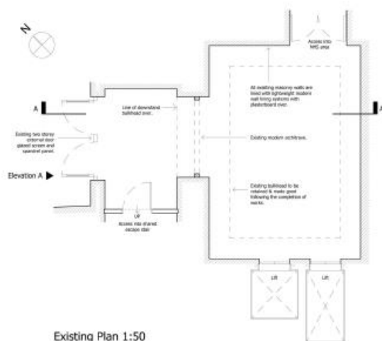
Existing Plan 1:50
