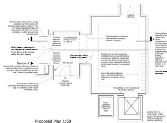
Proposed Plan 1:50
