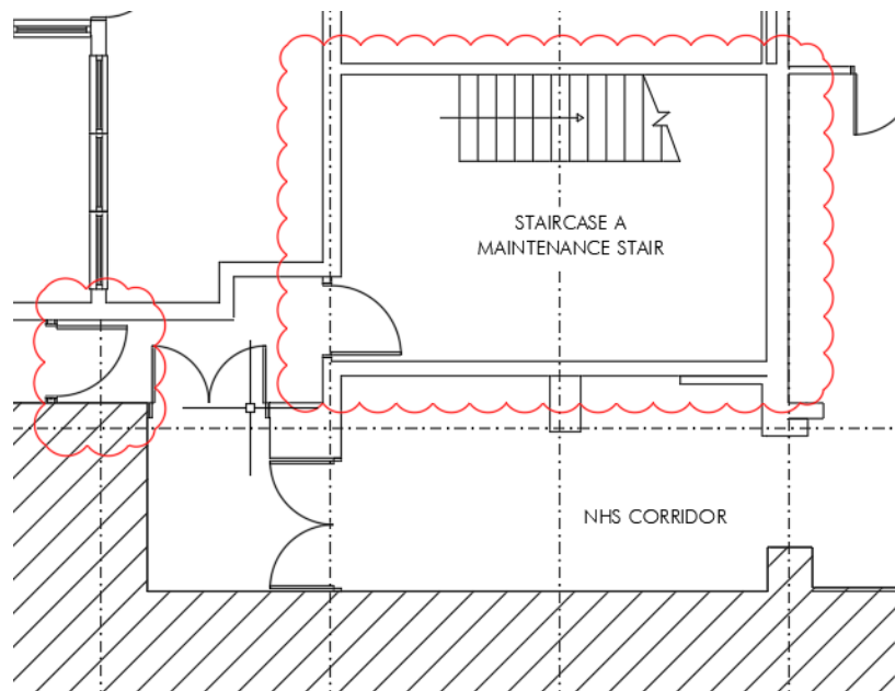
Extract of the ground floor plan showing the addition of a door (highlighted in red revision cloud)
