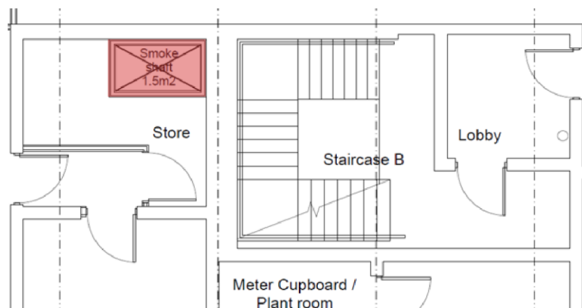
Location of the smoke vent for staircase B
