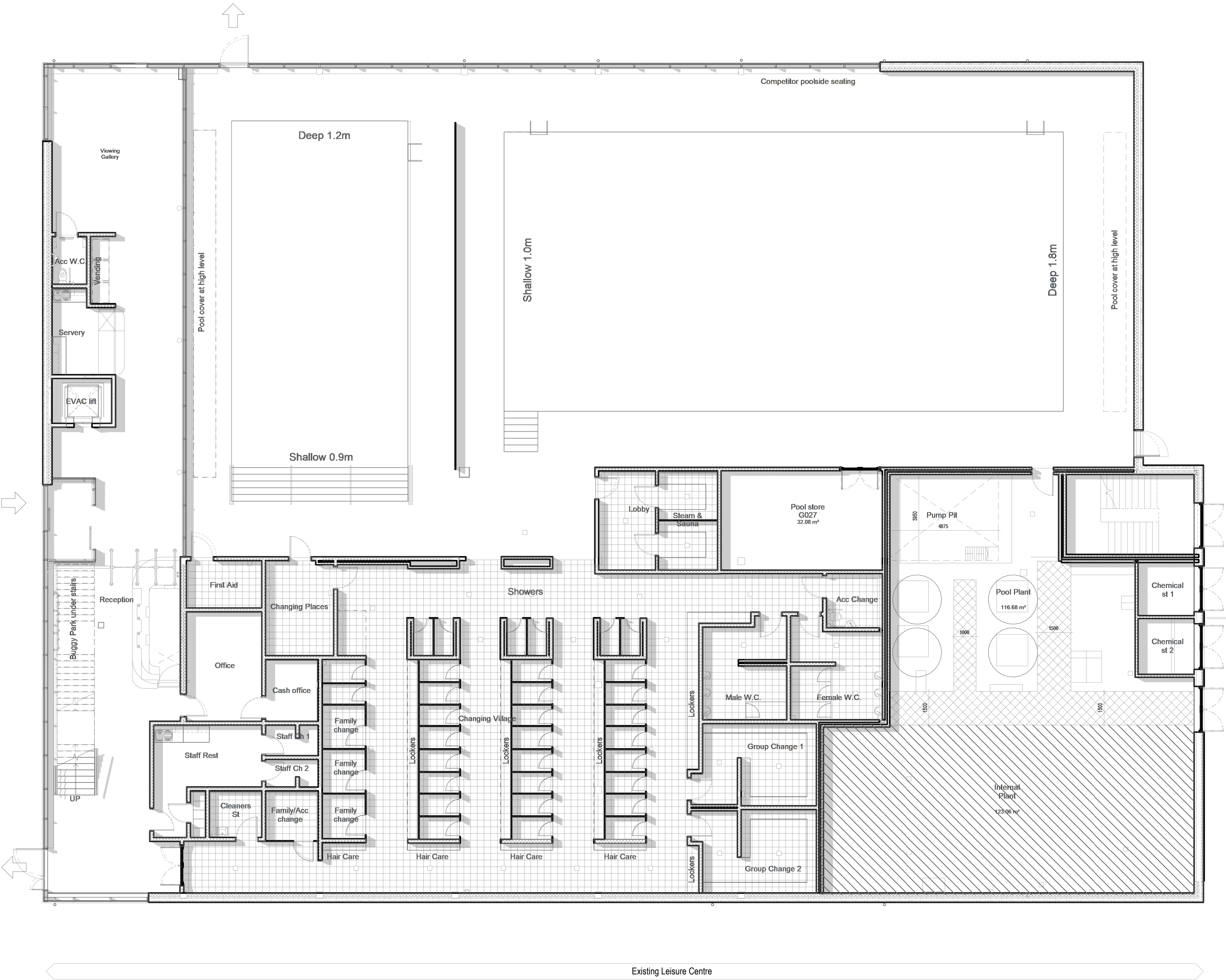
1 | (04)_Level 00 As Existing Layout Produced From Aedas As Built Drawings
