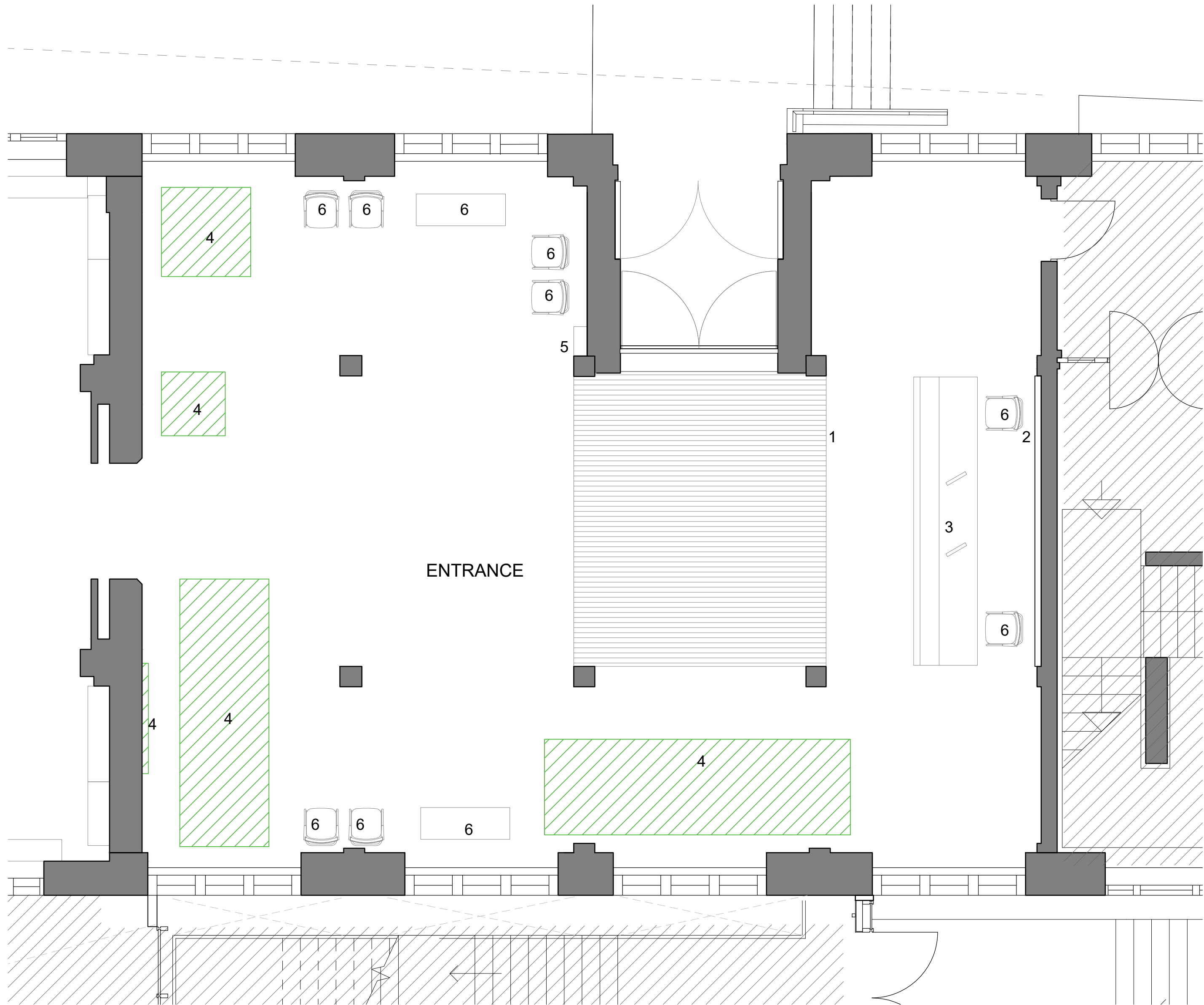
Ground Floor Proposed Plan - Entrance 1:50
