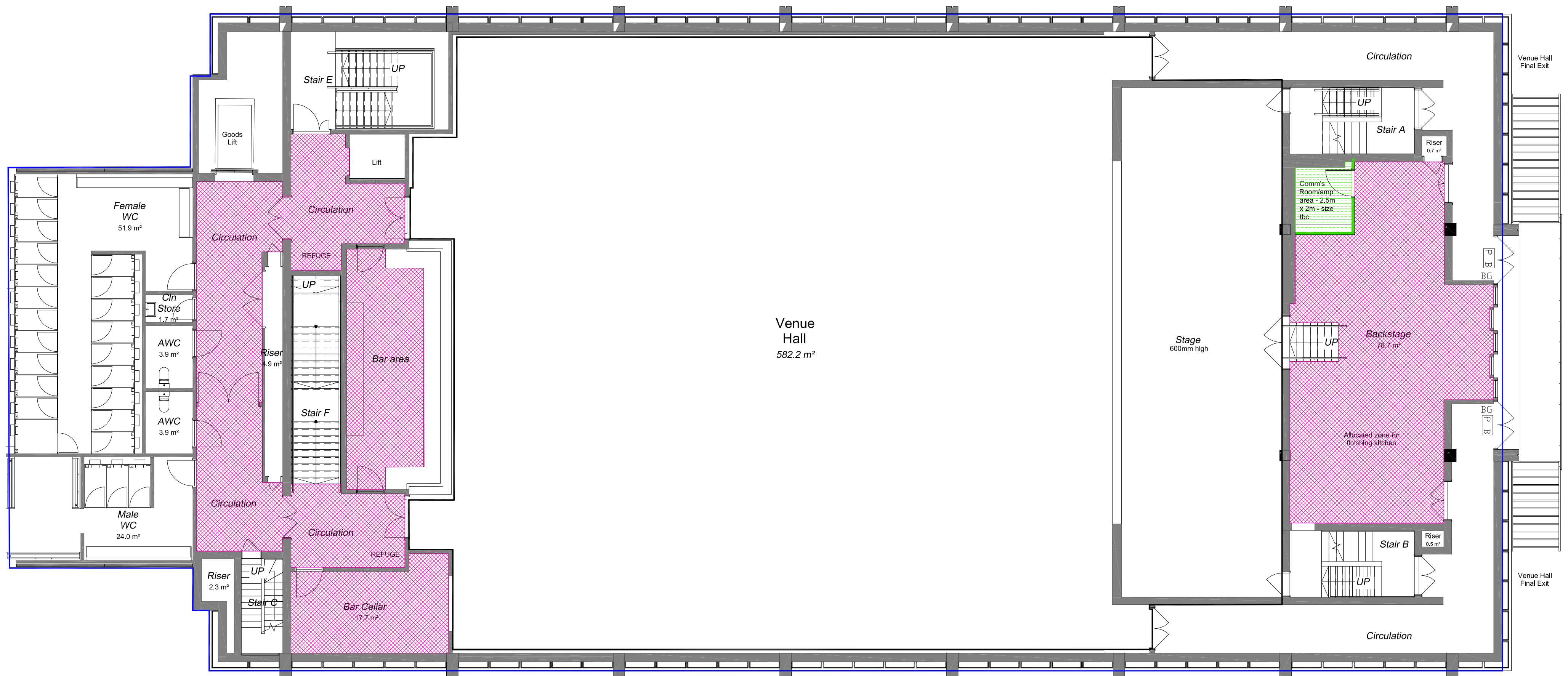
01 MEZZANINE FLOOR FINISHES PLAN Scale 1:100
