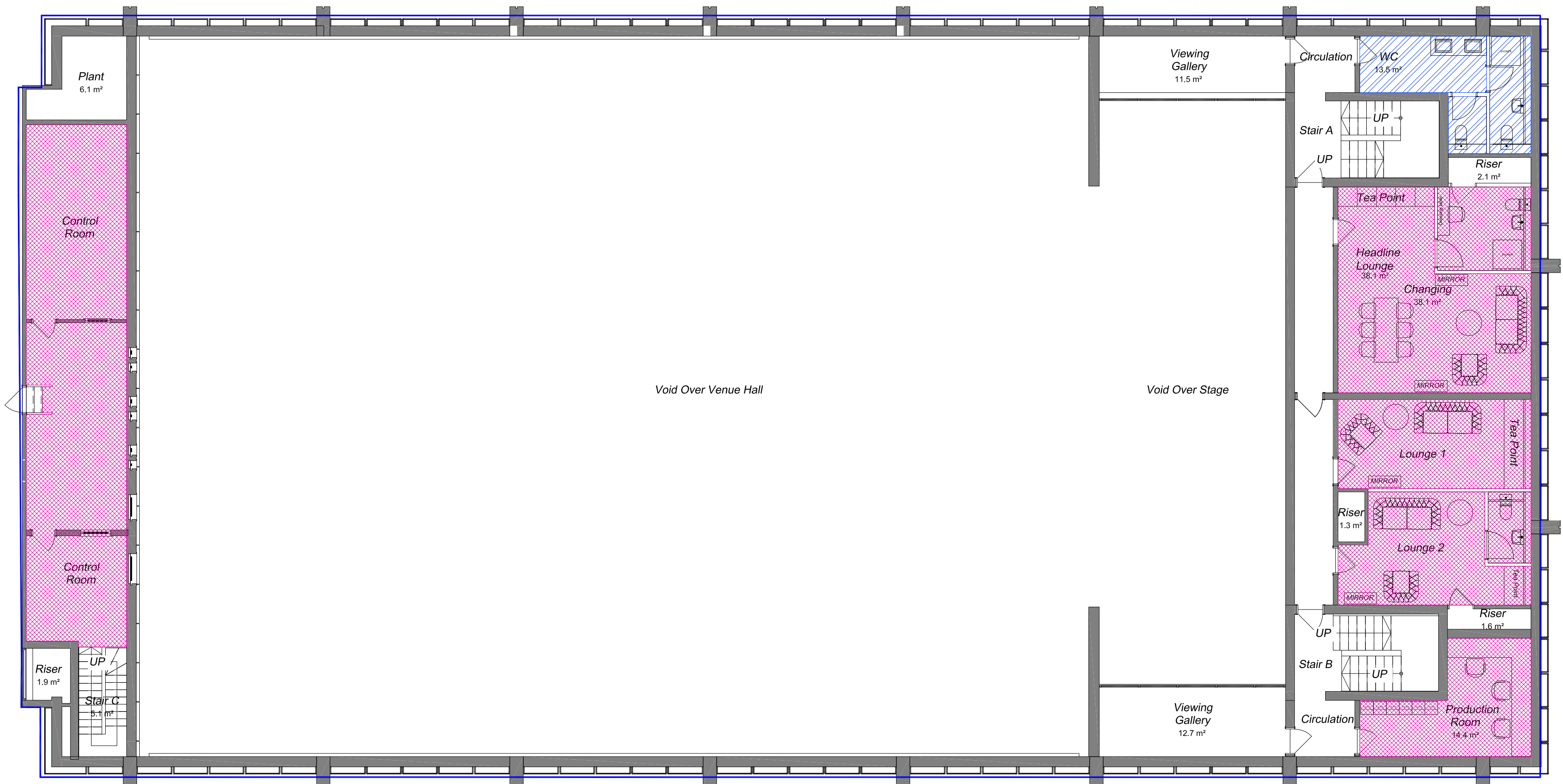
01 MEZZANINE FLOOR FINISHES PLAN Scale 1:100
