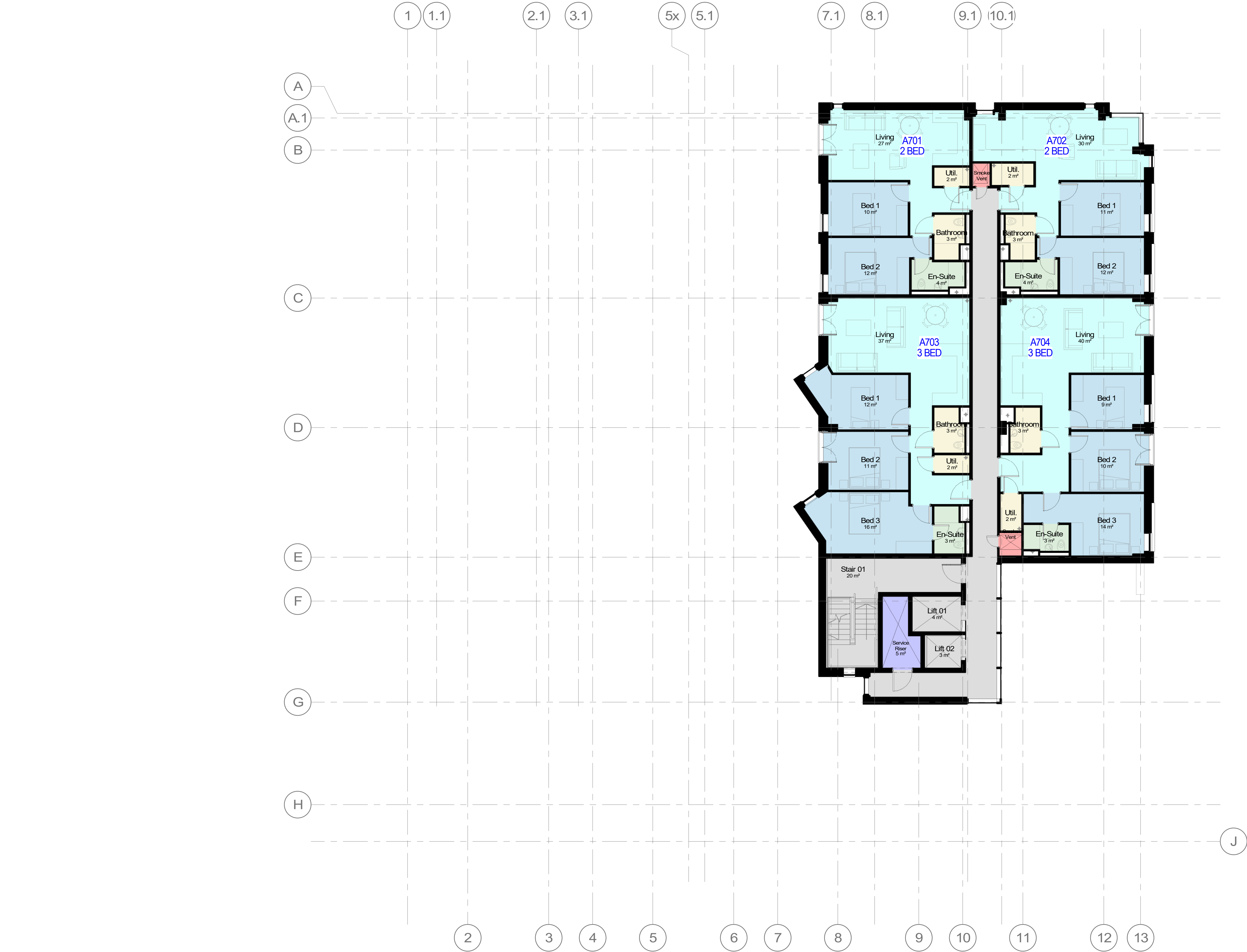
1 Seventh Floor GA Plan 1 : 100
