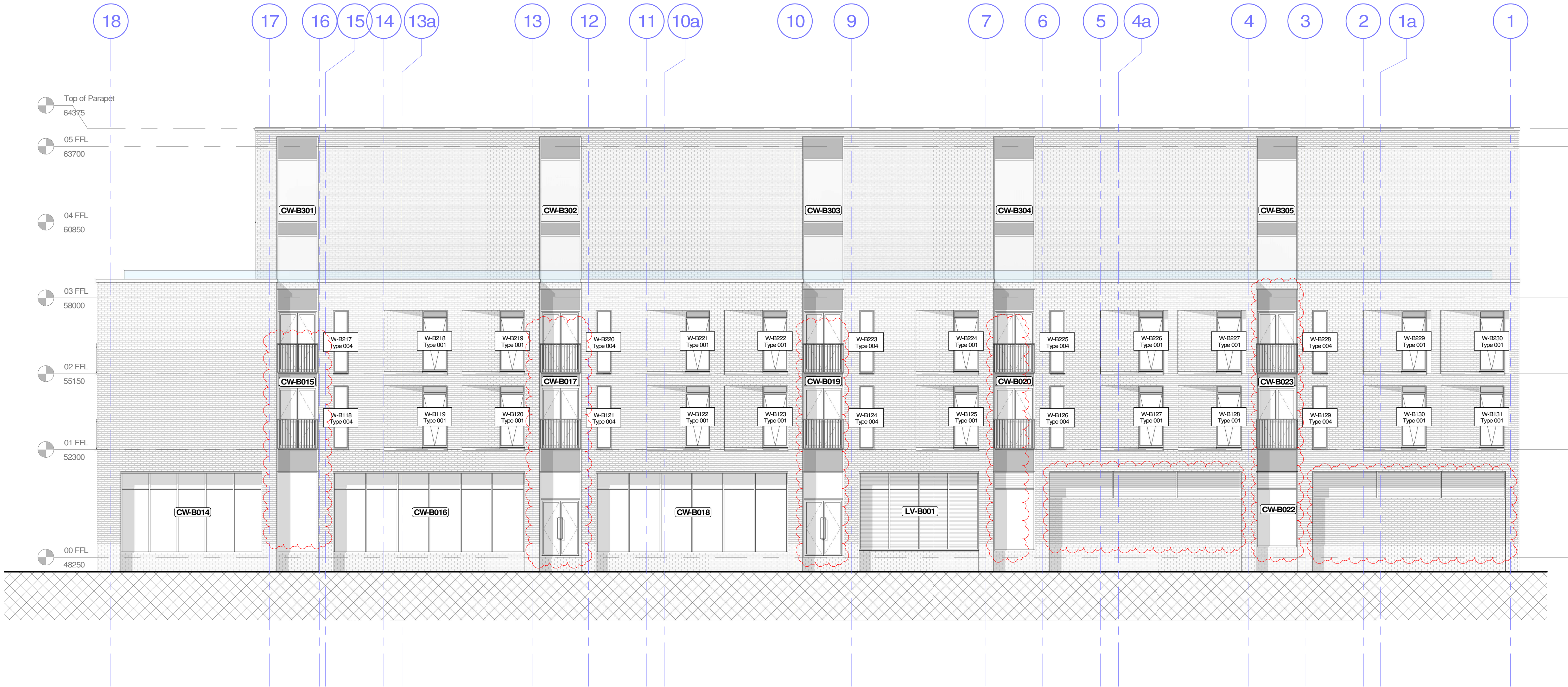
1 GA Elevation Bradley Street 1 : 100
