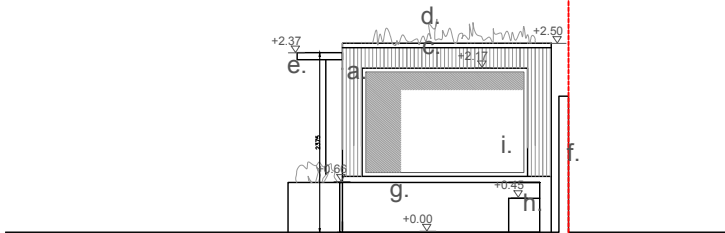
Elevation AA as proposed
