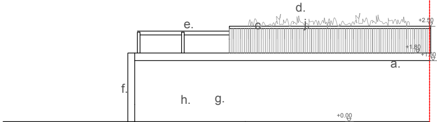
Elevation CC as proposed
