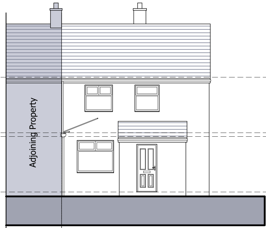
FRONT ELEVATION (South)
