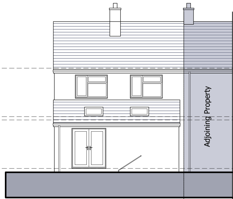
REAR ELEVATION (North)
