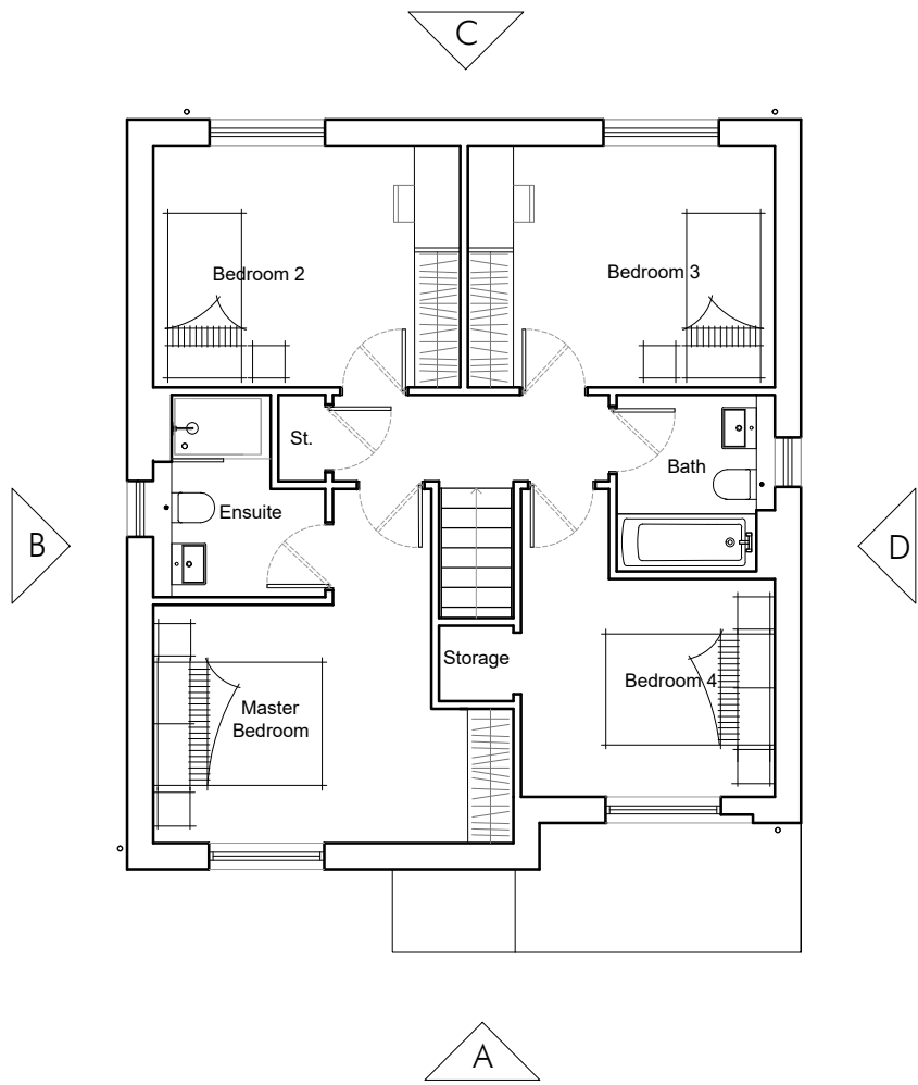
First Floor 62m²/672ft²
