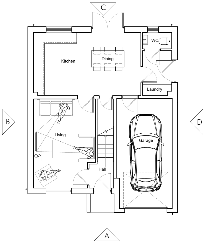
Ground Floor - ex Garage 48m²/518ft²
