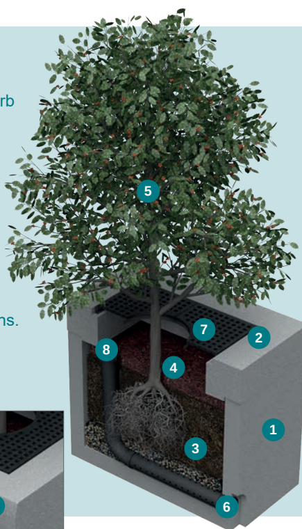
Figure 1 - The Hydro Biofilter™ Bioretention System
