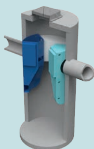
First Defense® Vortex Separator
