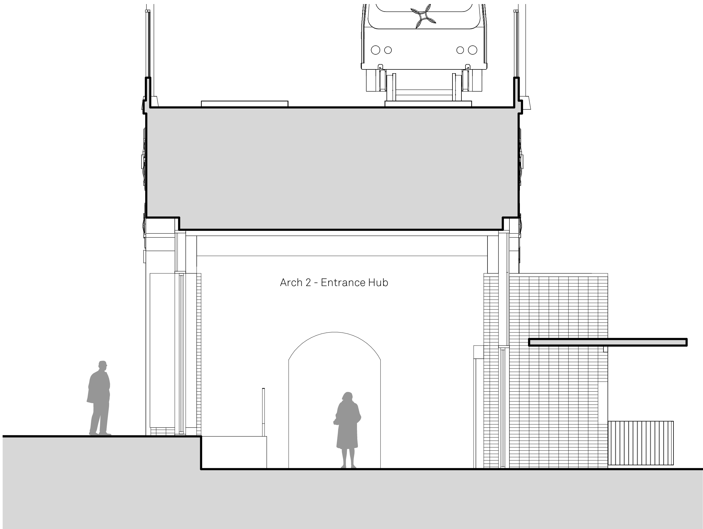
ARCH 02 Section A
