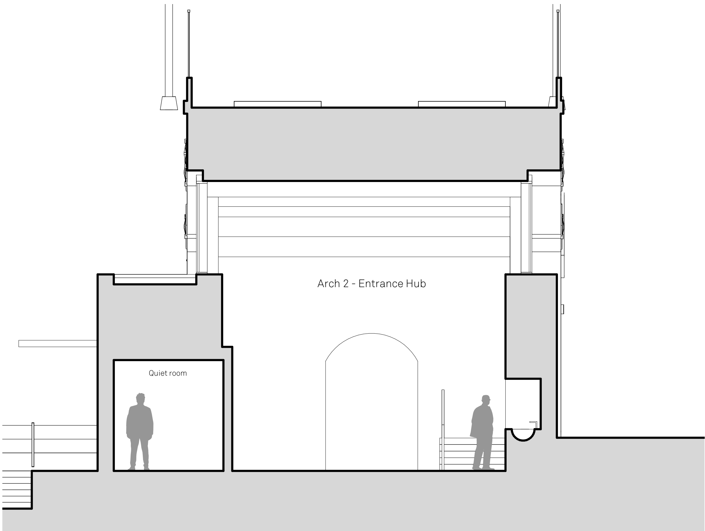
ARCH 02 Section B
