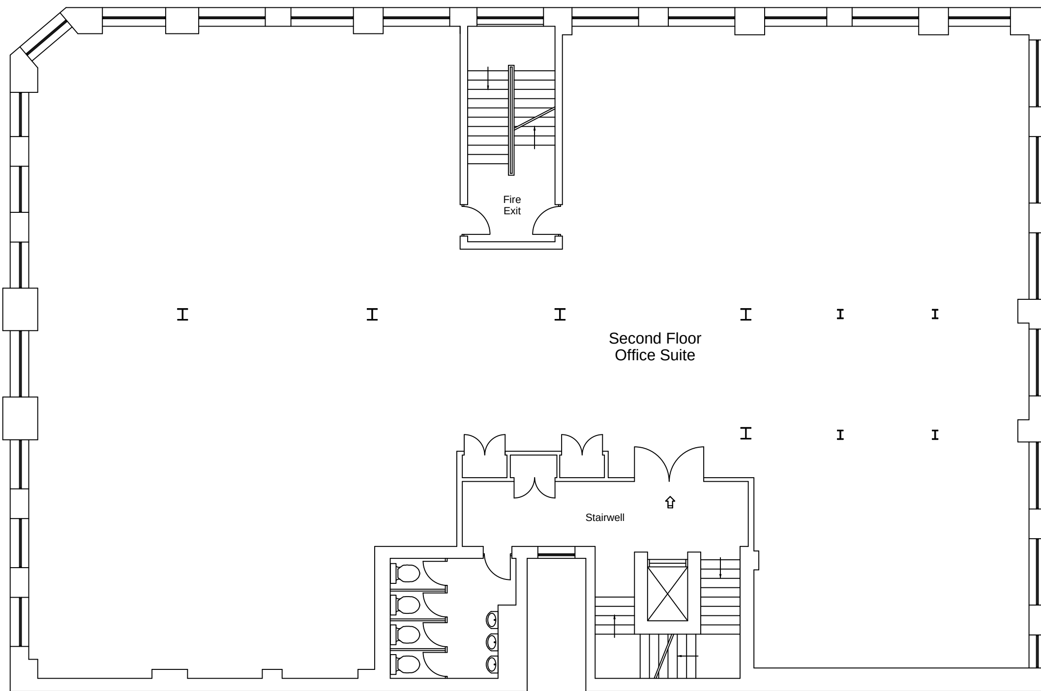
SECOND FLOOR
