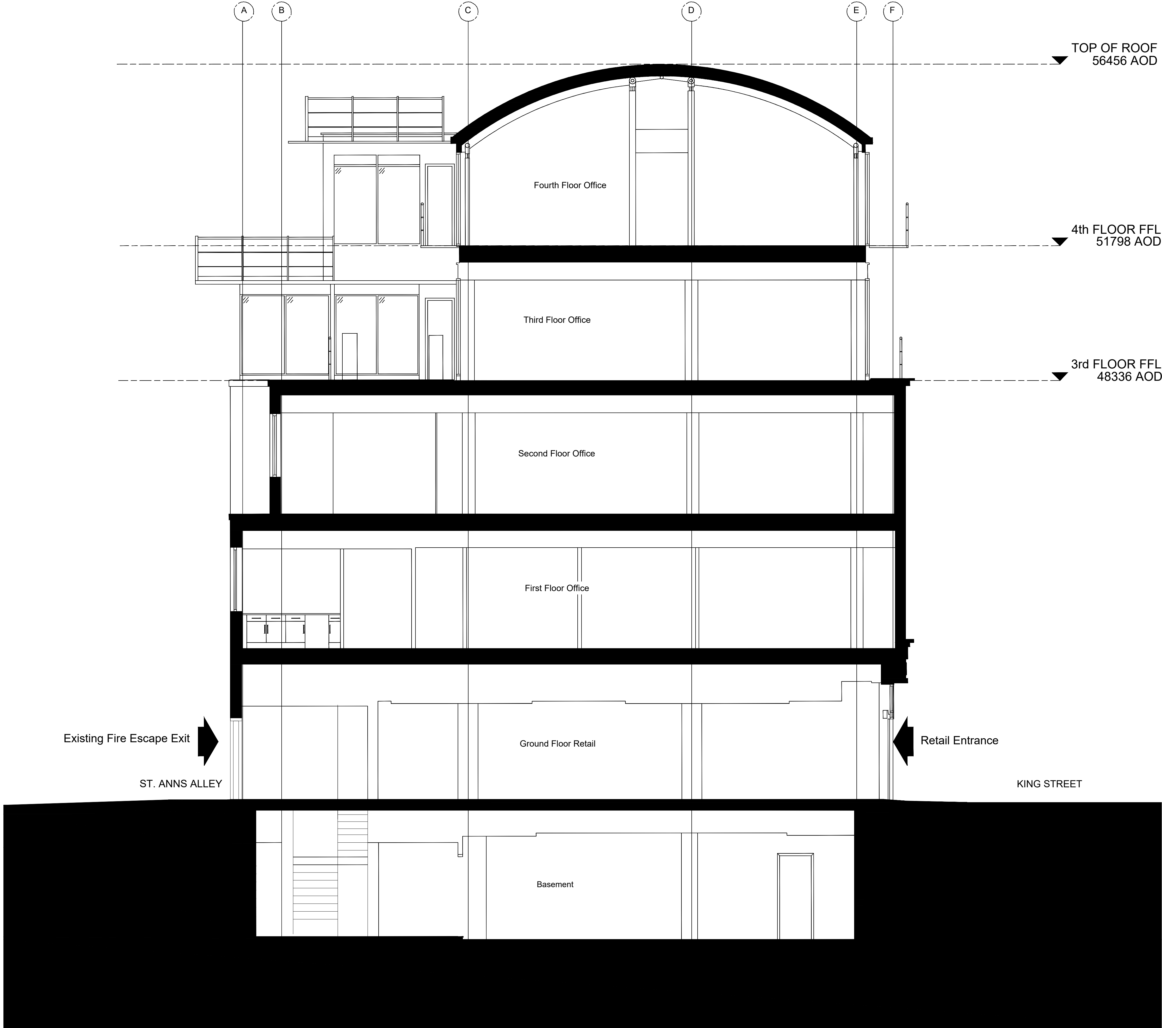
EXISTING BASEMENT BUILDING SECTION SCALE 1:50
