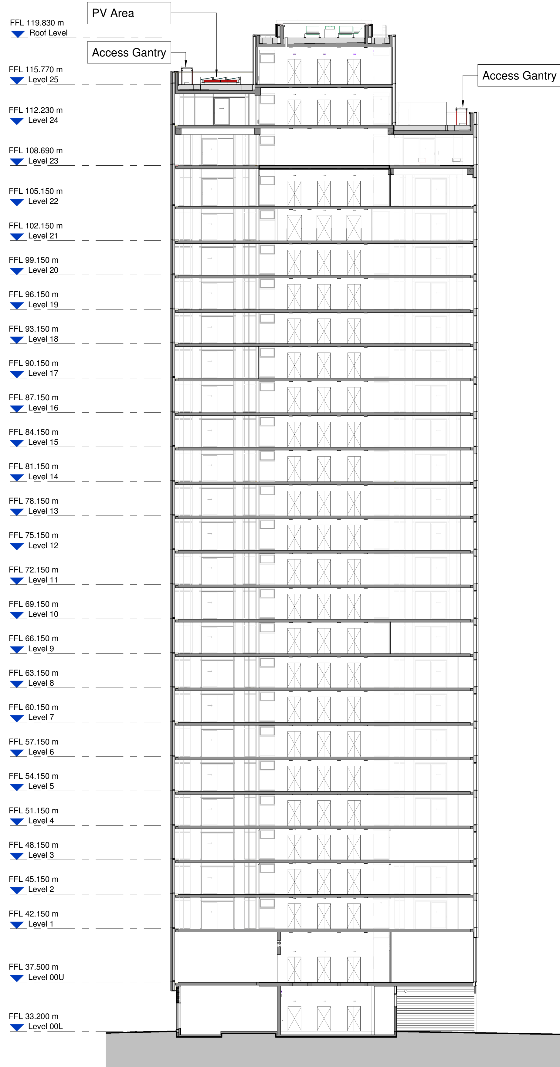
Section BB
