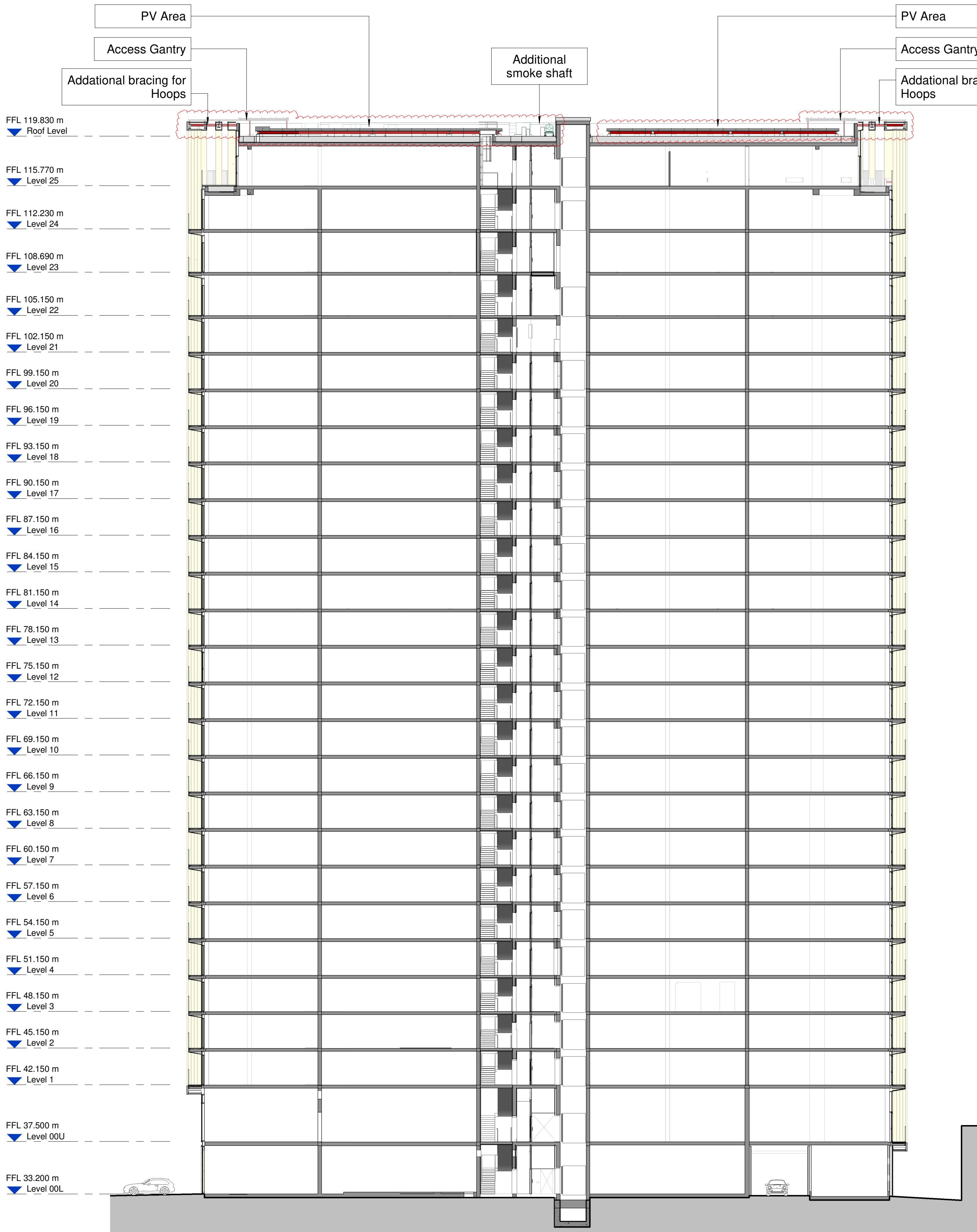
Section AA
