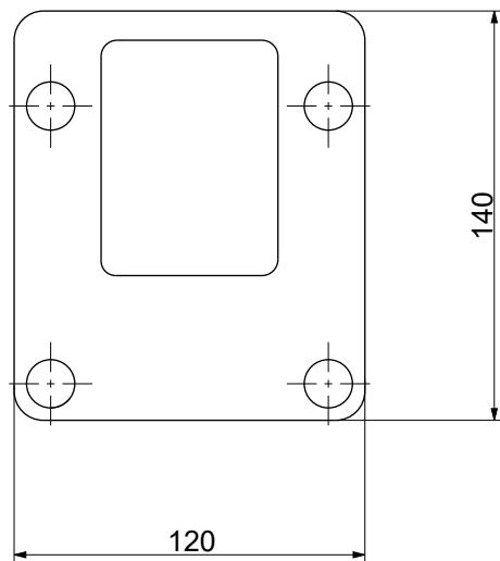
Baseplate Detail
