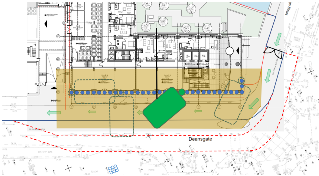
Indicative Logistics Layout for Piling Operations showing possible options for hoarding extensions
