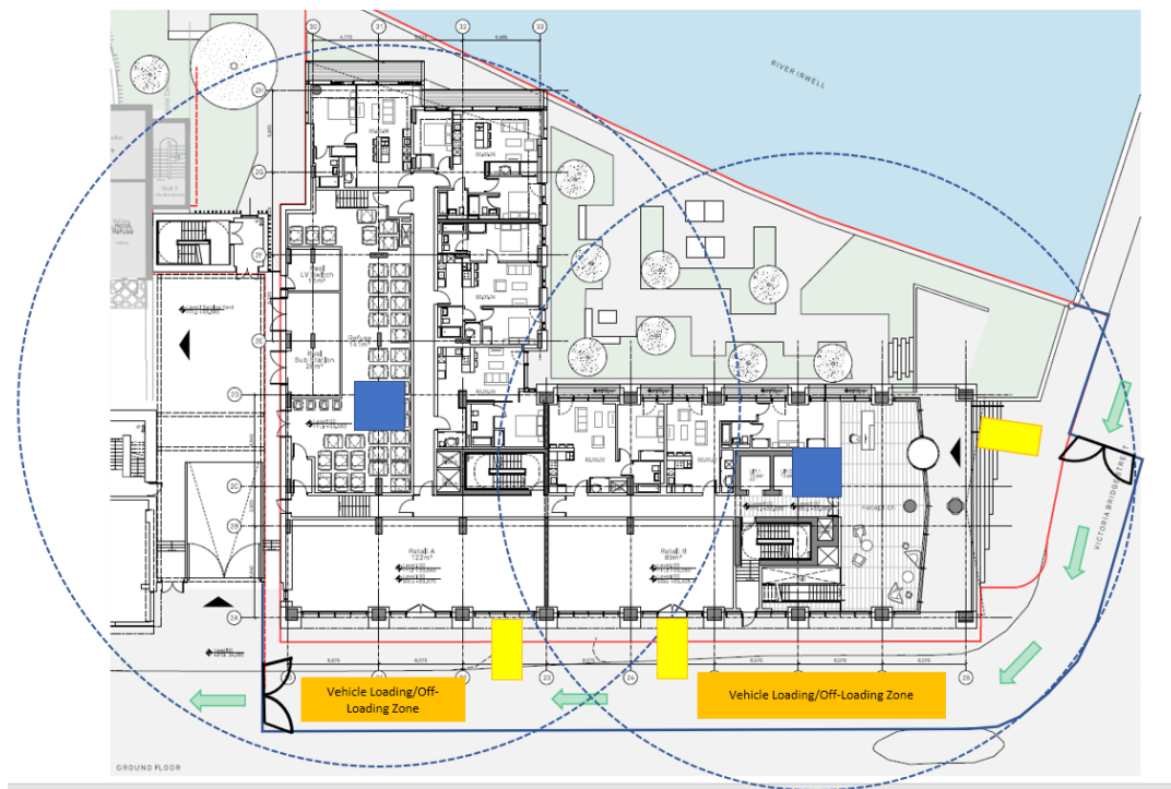
Indicative Logistics – tower cranes and hoists
