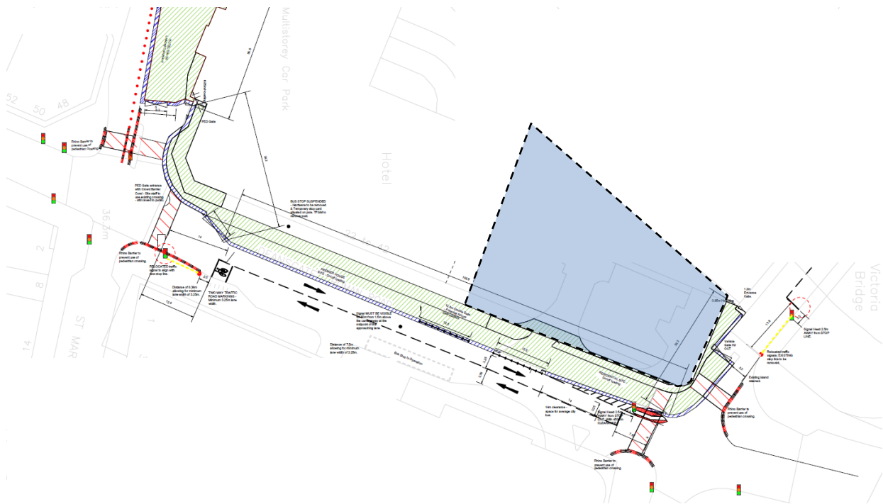
Site Hoarding Layout Plan with Gate Positions (combined development)
