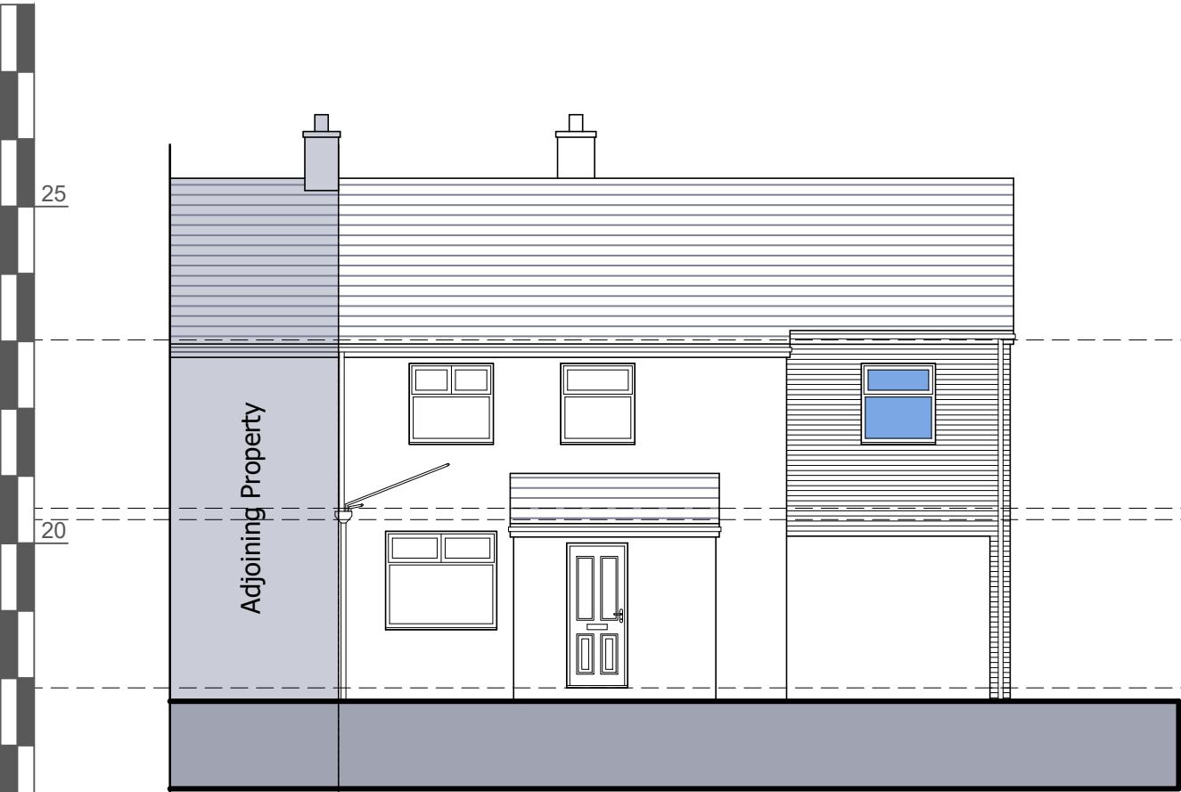
FRONT ELEVATION (South)
