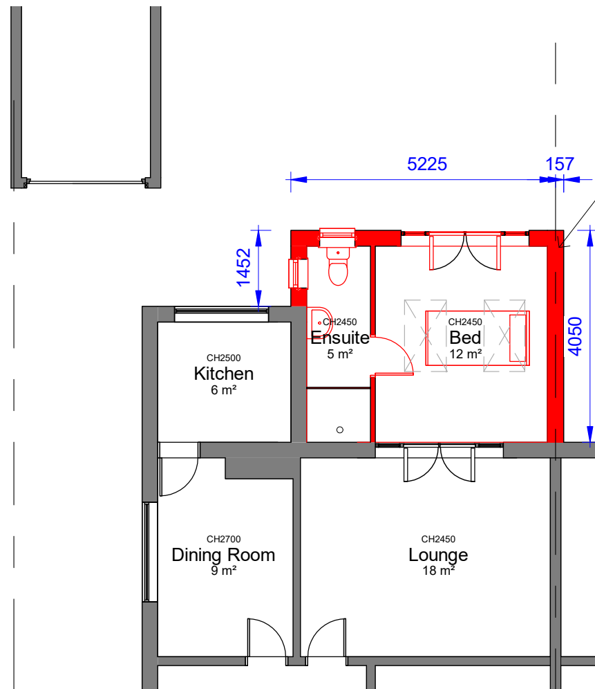
00-P-Ground Floor 1 : 100
