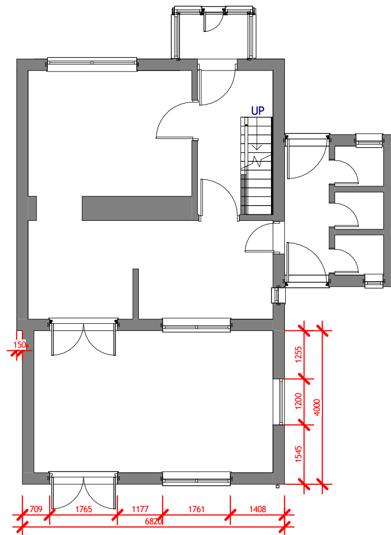
1 Ground Floor proposed 1 : 100
