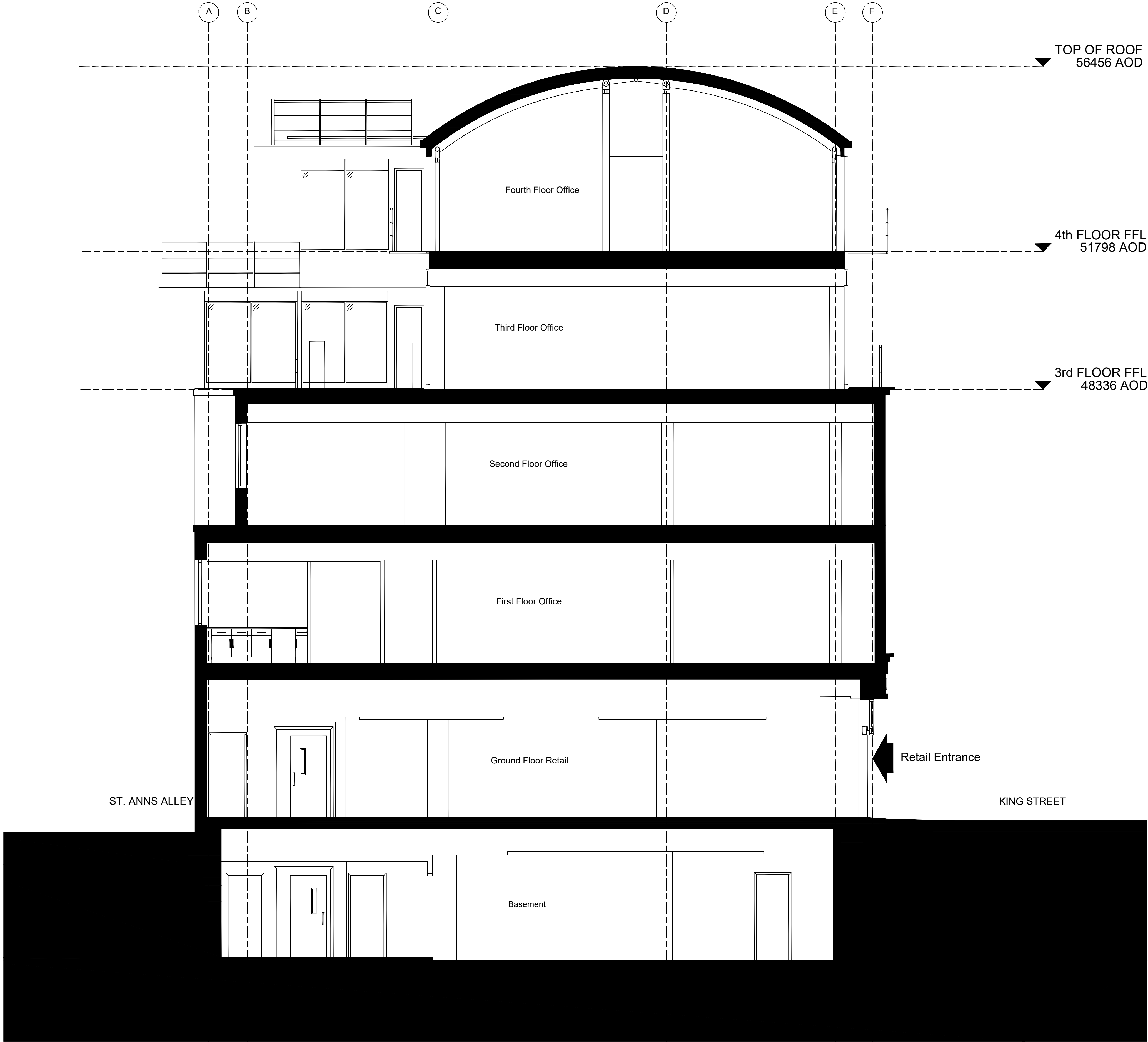
EXISTING GROUND FLOOR RETAIL UNIT SECTION SCALE 1:50
