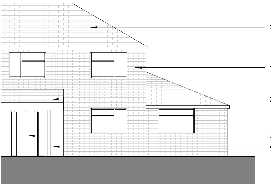
Proposed Elevation North no. 10 1 : 100
