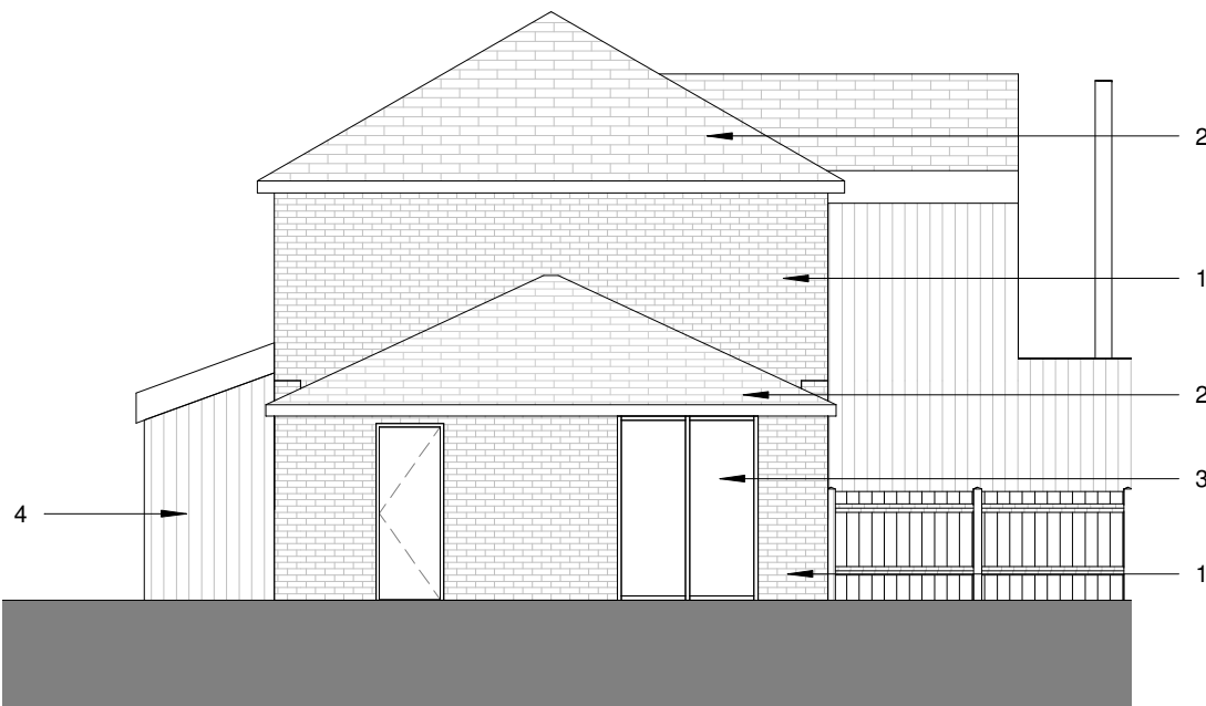
Proposed Elevation West no. 10 1 : 100
