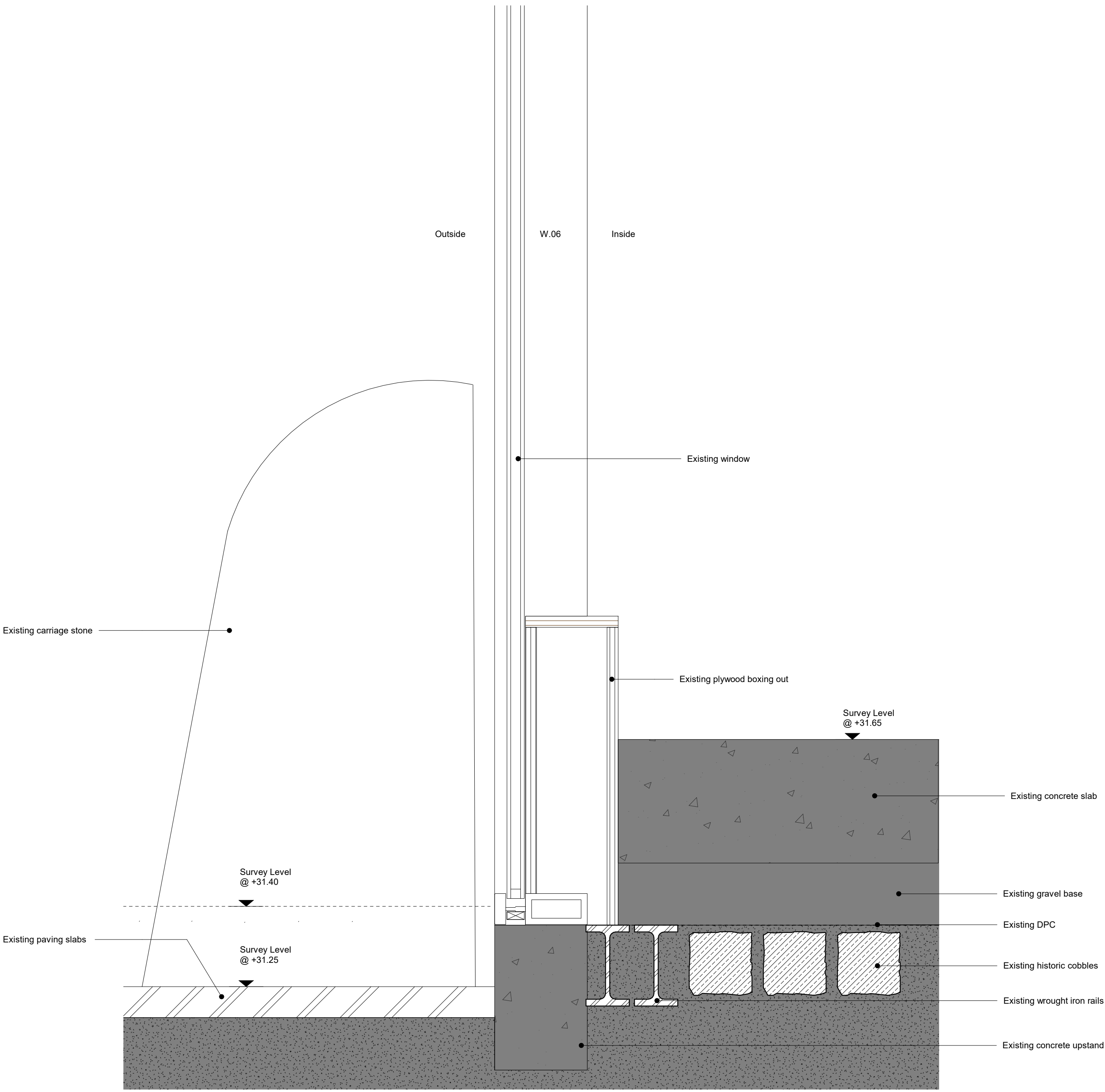
02 Detail Section 02 W.06 Existing 1 : 5 @ A1
