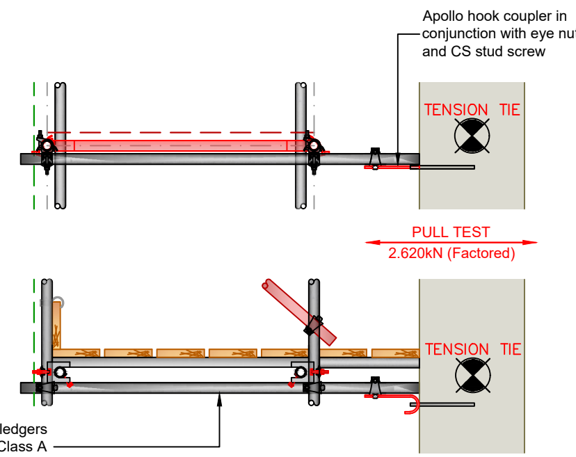
PREFABRICATED TRANSOM HOOK TIE DETAIL scale 1:25
