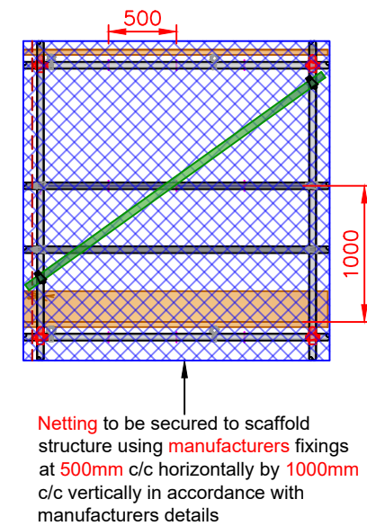
TYPICAL NETTING DETAIL scale 1:50
