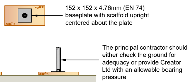
FOUNDATION DETAIL 225 x 38 x 450mm (BS EN 2482) Scaffold Board Solepad Scale - 1:25
