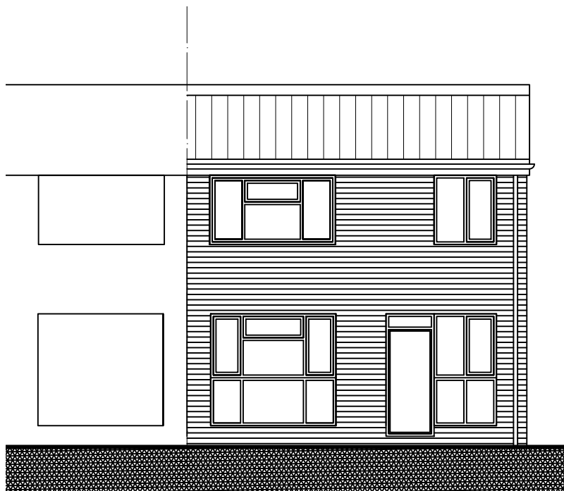
Existing Elevation 2
