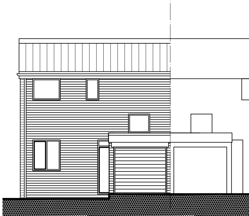
Existing Elevation 1
