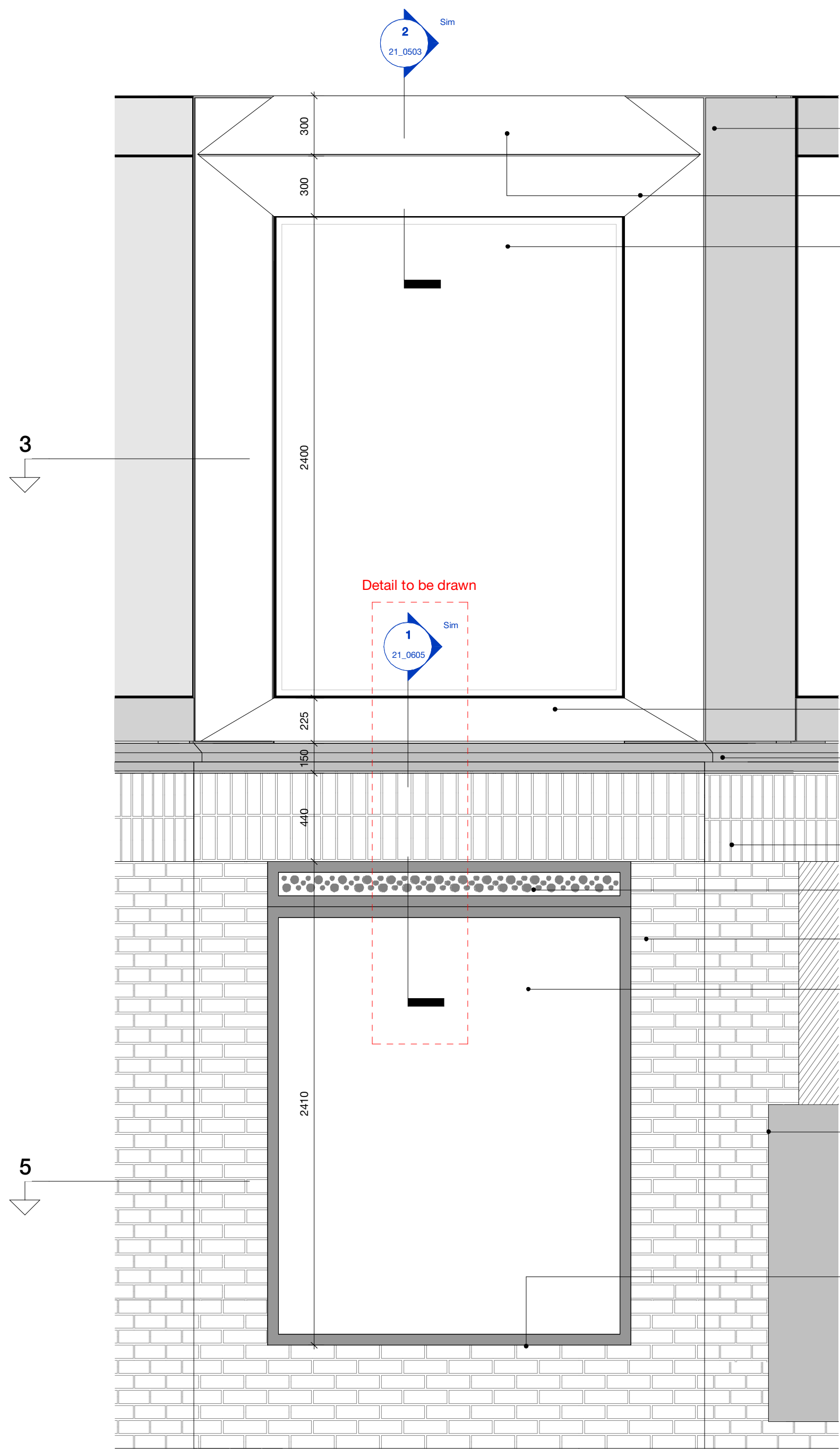
2 Mock-Up Panel - Picture Windows - Elevation
