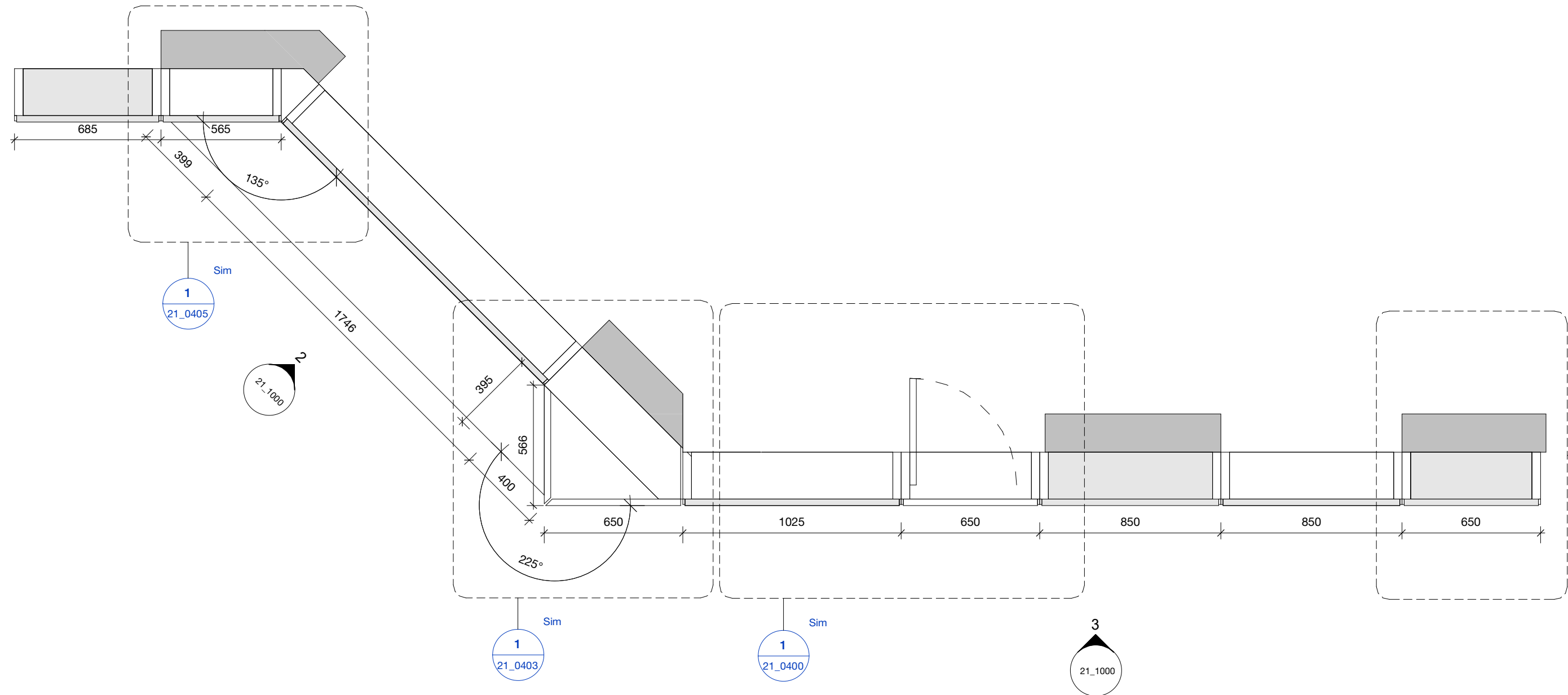
4 Mock-Up Panel - Unitised Facade - Plan
