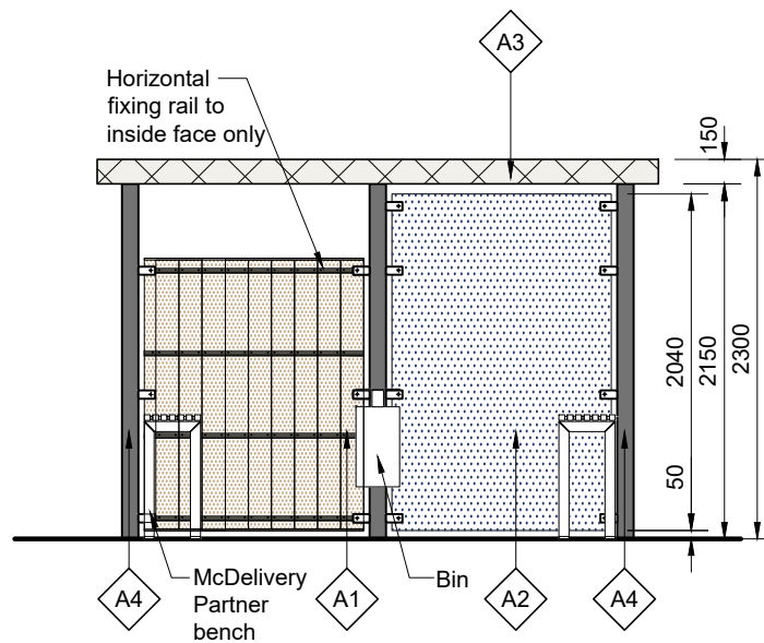
FRONT ELEVATION
