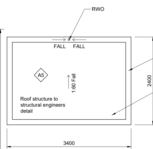
ROOF PLAN
