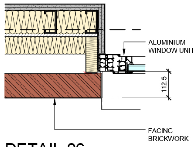
DETAIL 06
