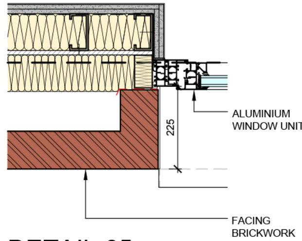
DETAIL 05
