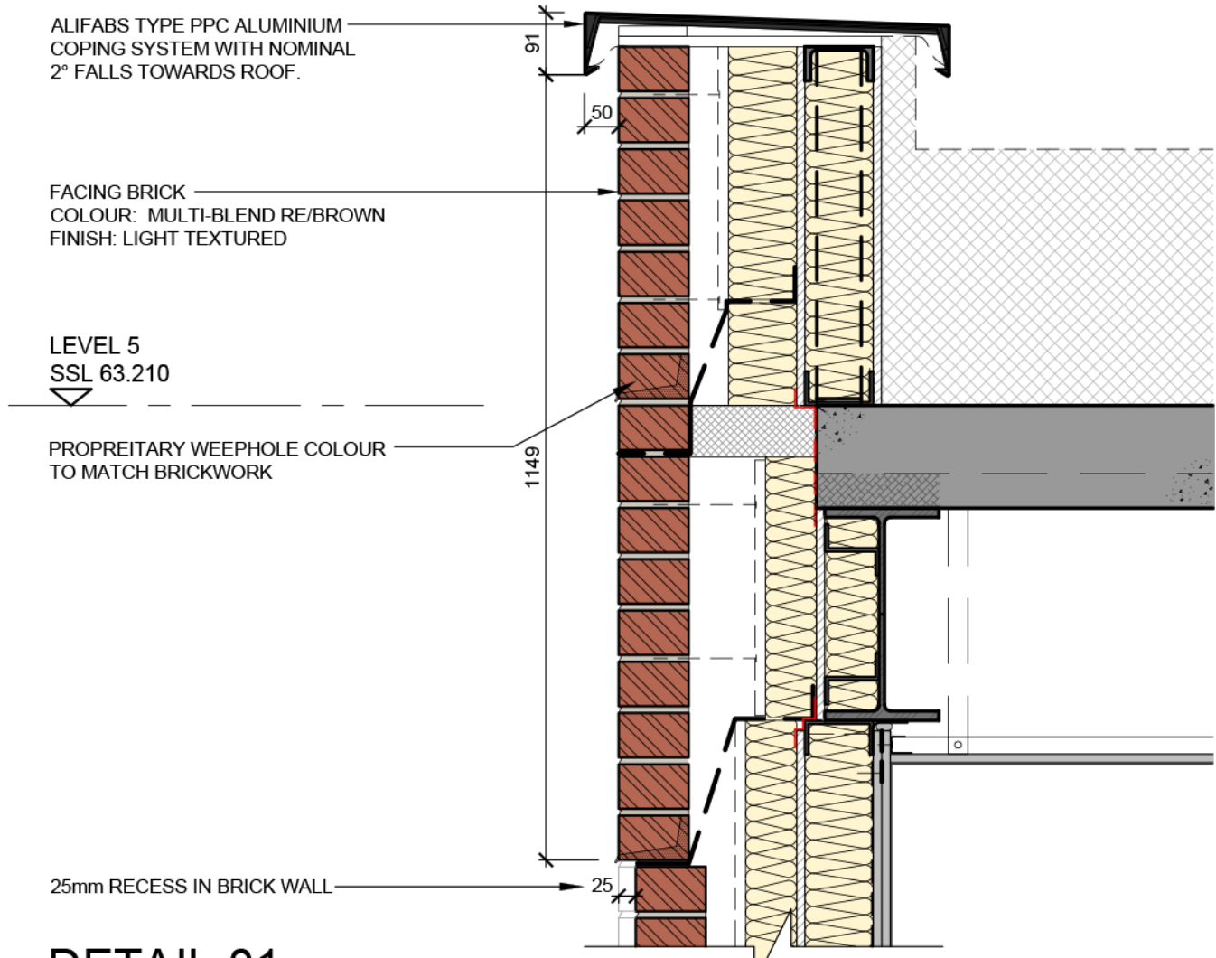
DETAIL 01
