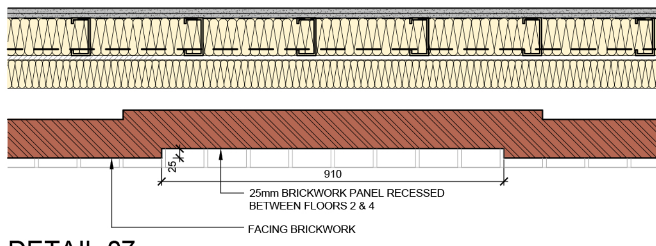
DETAIL 07
