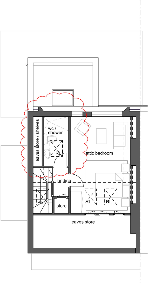
Proposed Second Floor
