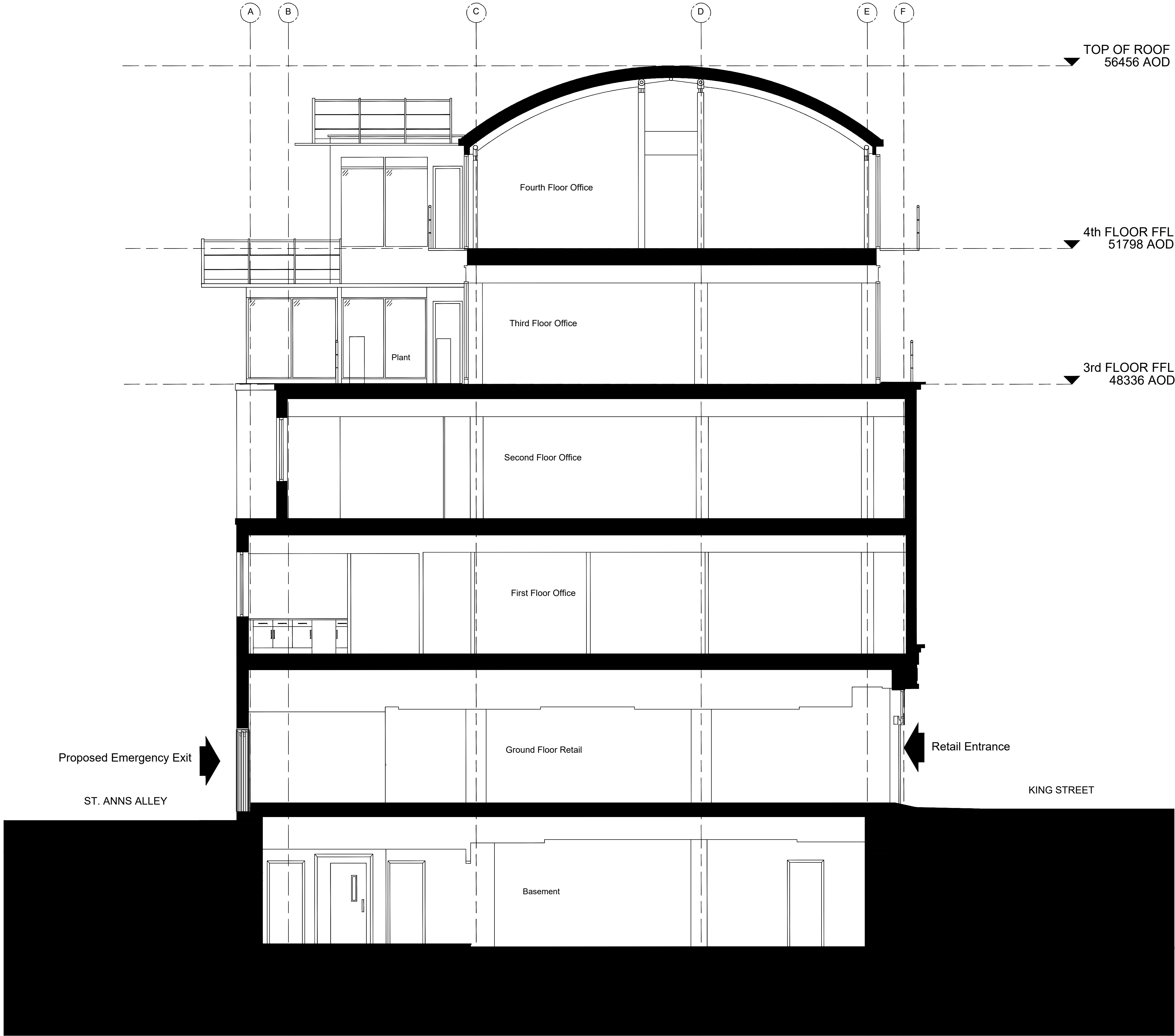
PROPOSED GROUND FLOOR BUILDING SECTION SCALE 1:50
