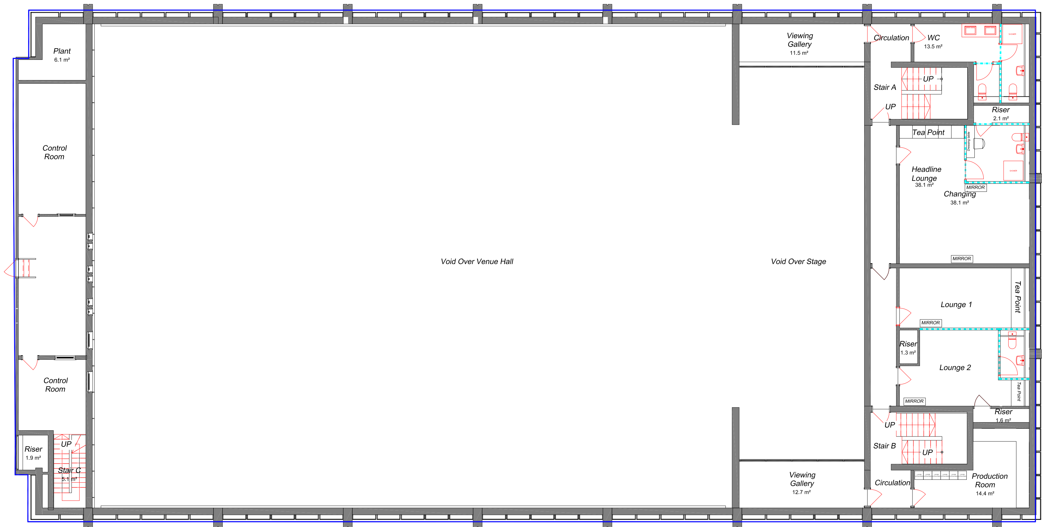
01 MEZZANINE PARTITION PLAN Scale 1:100
