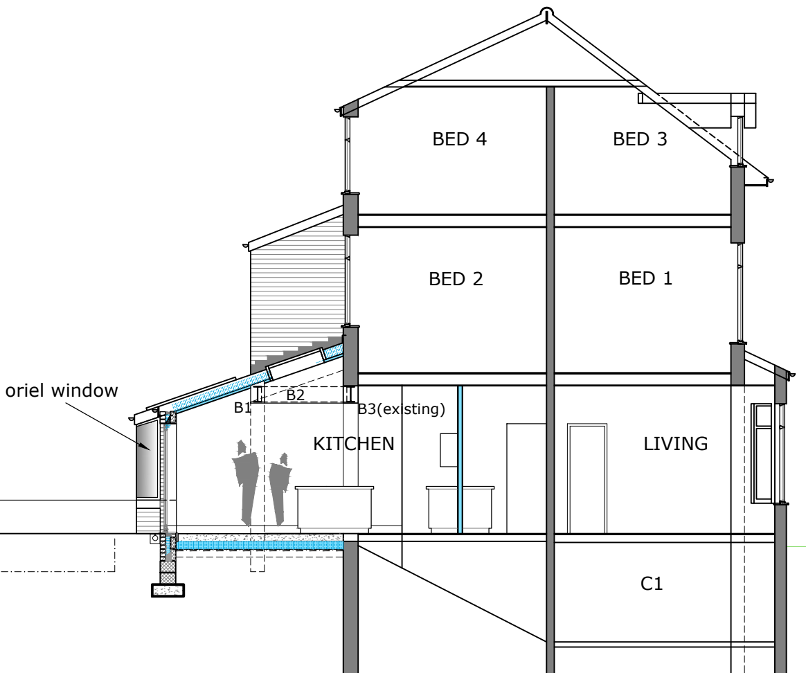
CROSS SECTION
