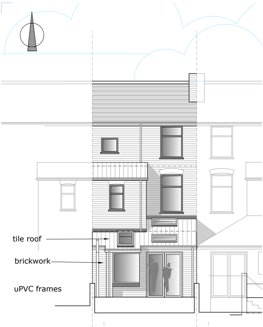
SOUTH ELEVATION
