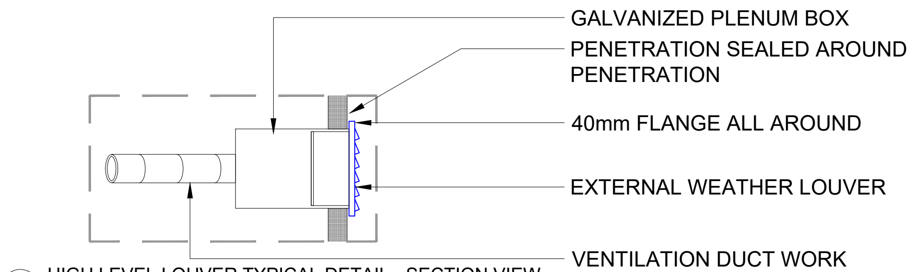
02 HIGH LEVEL LOUVER TYPICAL DETAIL - SECTION VIEW Scale: 1:20@A1
