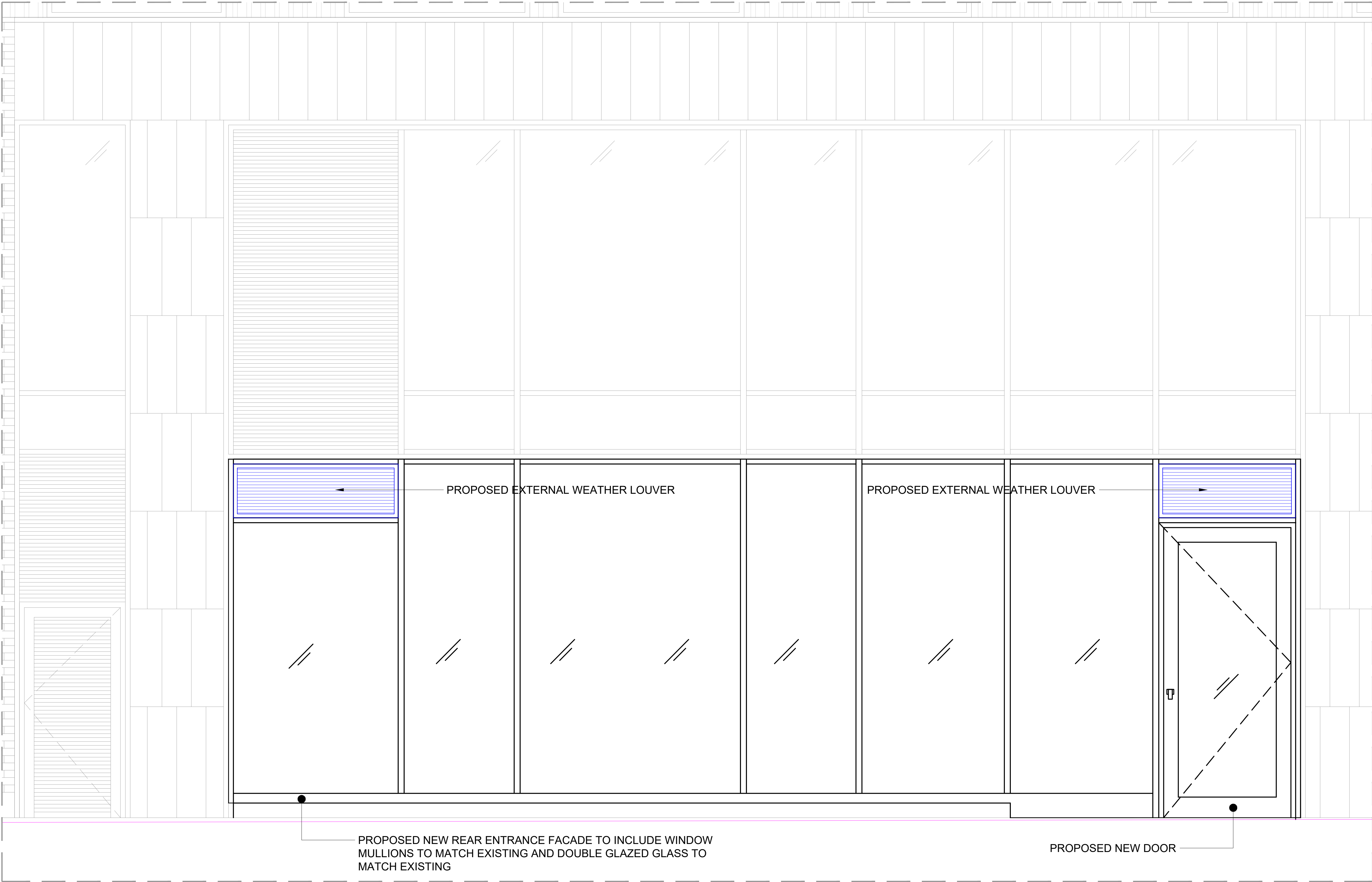
01 PROPOSED DETAILED MUSEUM STREET ELEVATION - OPTION 1 Scale: 1:20@A1
