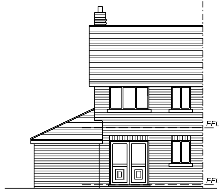
East Elevation
