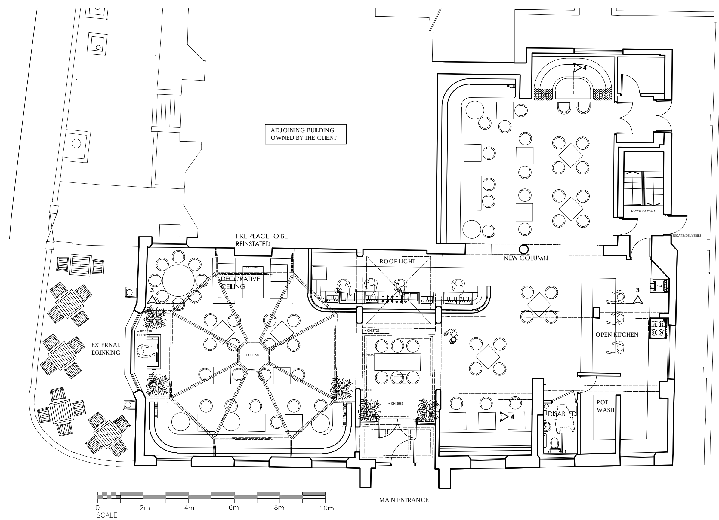
KEY PLAN (1:100)
